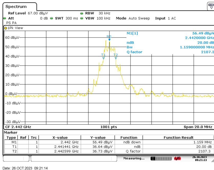
20dB Bandwidth Test Plot
