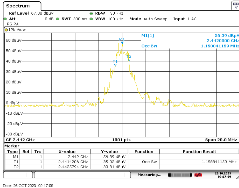
99% Bandwidth Test Plot
