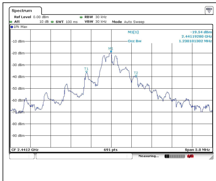
Channel: 2441 MHz
