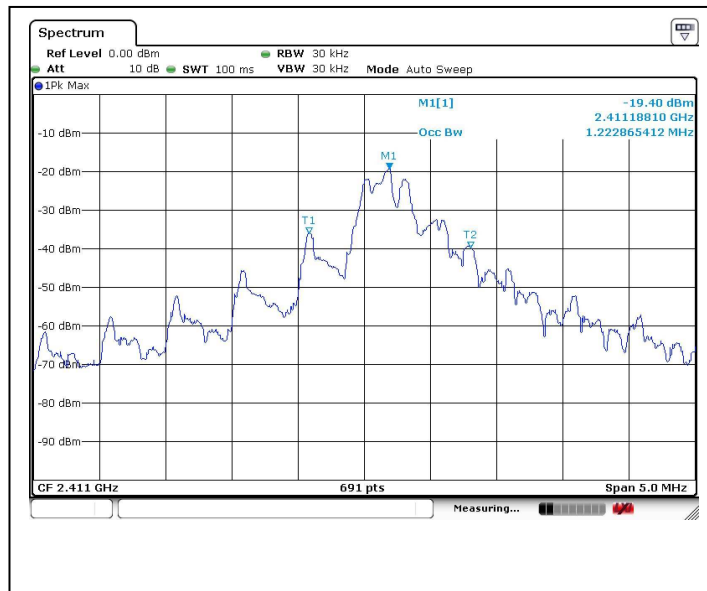
Channel: 2411 MHz
