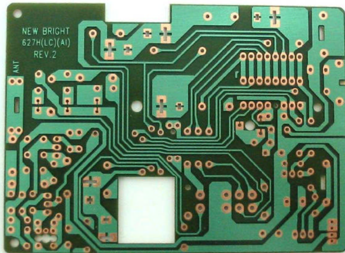
Model : 6277H(49M) Soldering side
