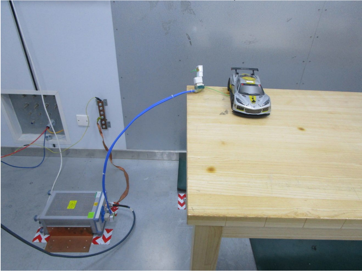
AC Conducted Power Setup
