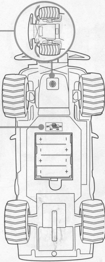
ON/OFF Switch
