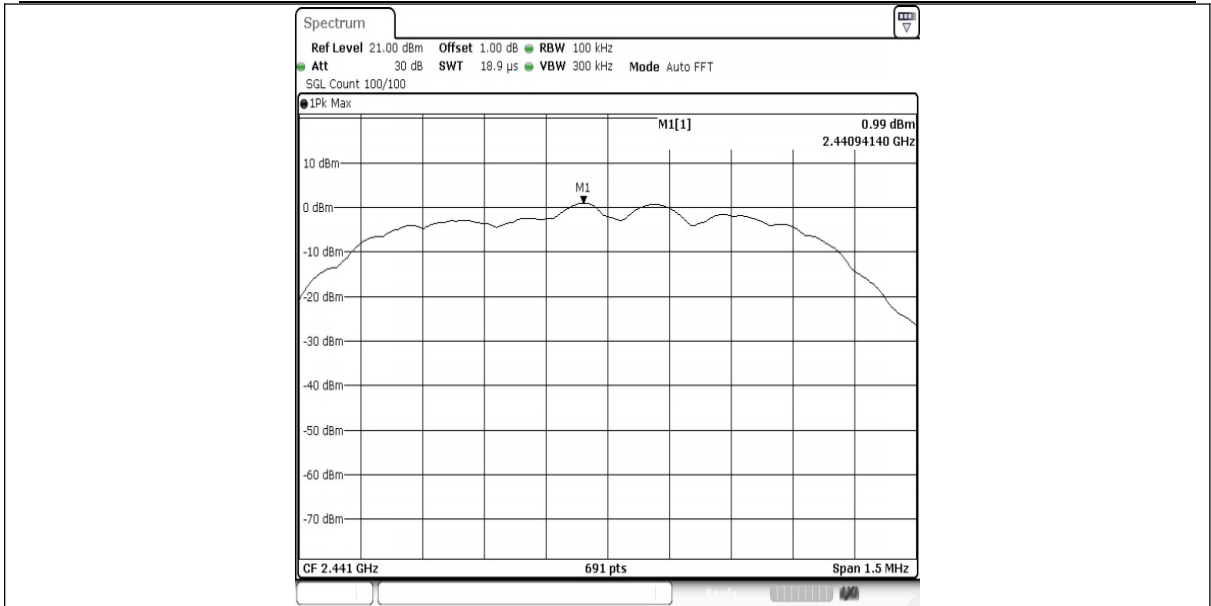
2DH5-Ant1-2441-0~Reference-PASS
