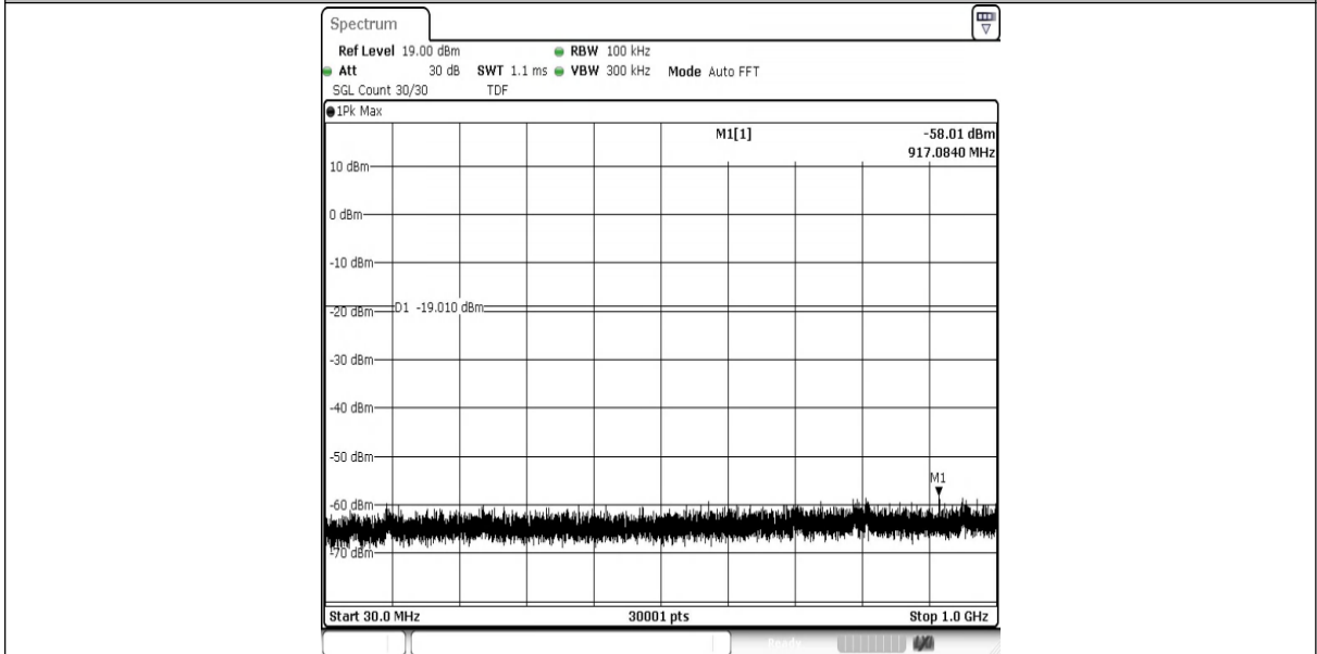
2DH5-Ant1-2441-30~1000-PASS
