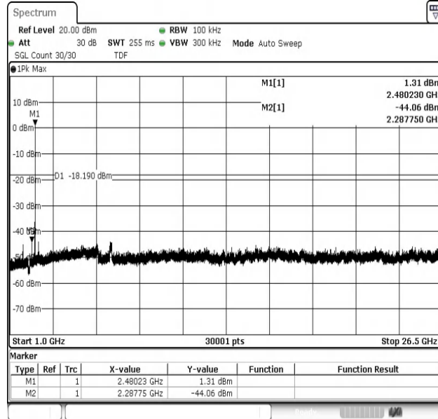
DH5-Ant1-2480-1000~26500-PASS
