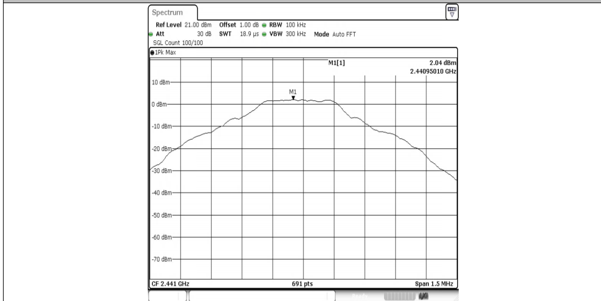
DH5-Ant1-2441-0~Reference-PASS
