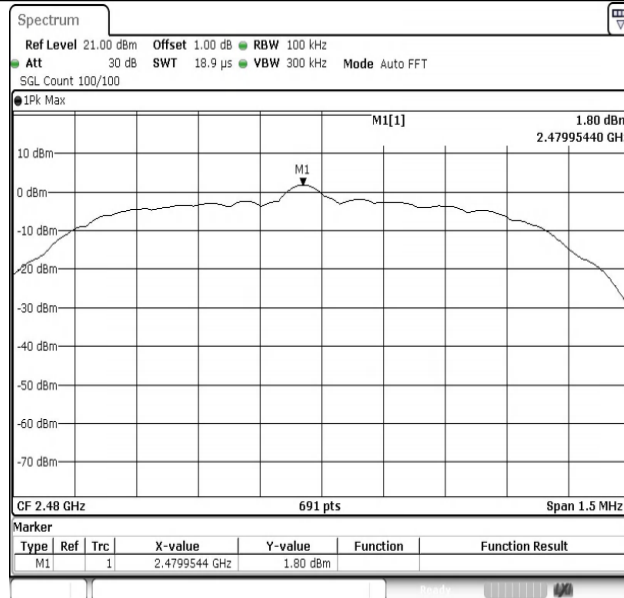
2DH5-Ant1-2480-0~Reference-PASS
