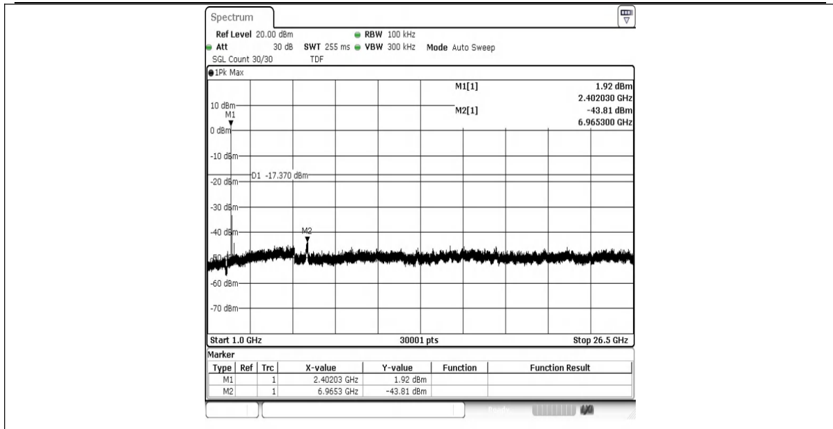
DH5-Ant1-2402-1000~26500-PASS
