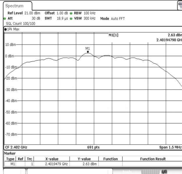
2DH5-Ant1-2402-0~Reference-PASS
