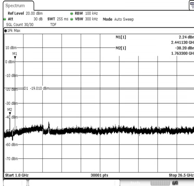
2DH5-Ant1-2441-1000~26500-PASS
