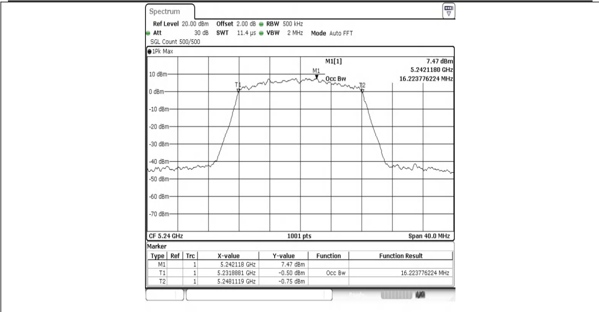
11A-Ant1-5240
