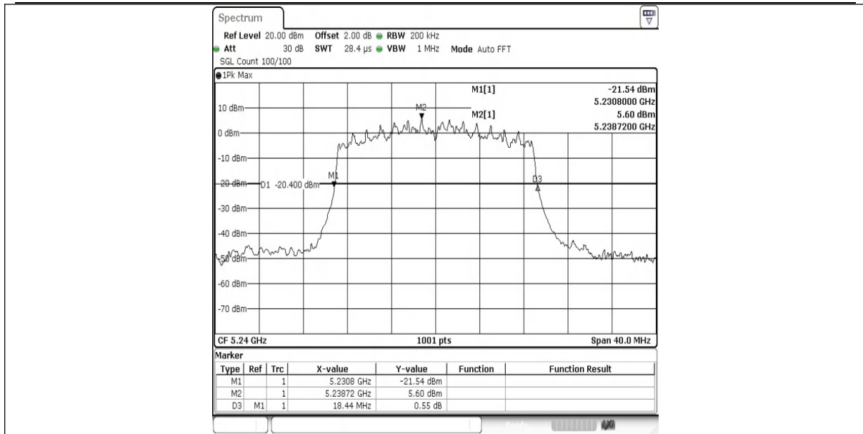
11N20SISO-Ant1-5240
