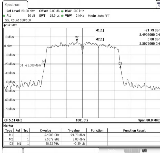
11N40SISO-Ant1-5510
