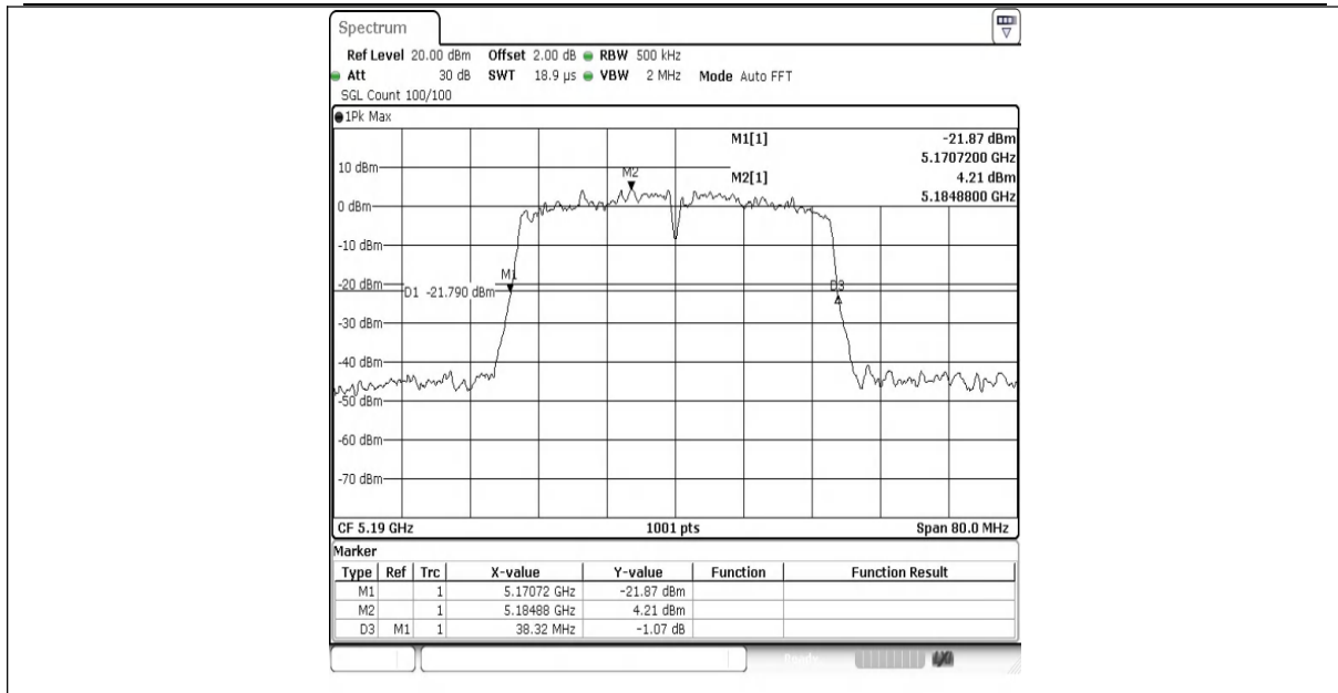
11N40SISO-Ant1-5190
