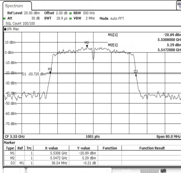
11N40SISO-Ant1-5550
