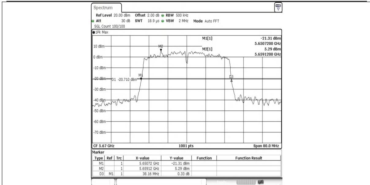
11N40SISO-Ant1-5670
