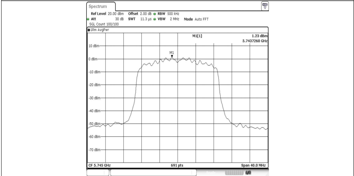
11N20SISO-Ant1-5745-PASS
