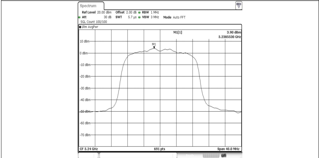
11N20SISO-Ant1-5240-PASS
