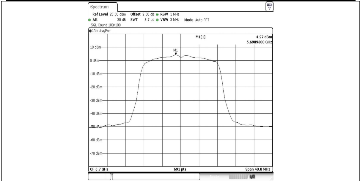
11A-Ant1-5700-PASS
