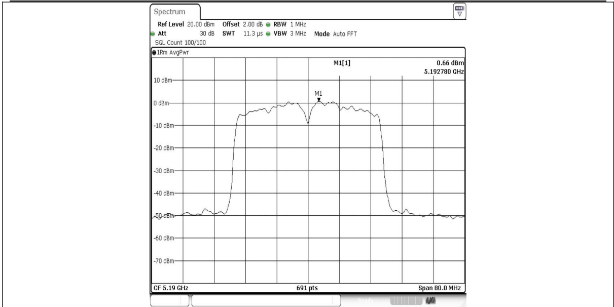
11N40SISO-Ant1-5190-PASS
