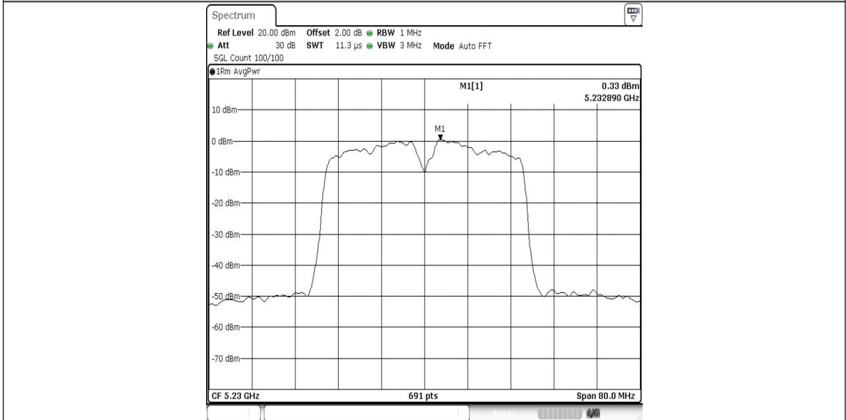
11N40SISO-Ant1-5230-PASS
