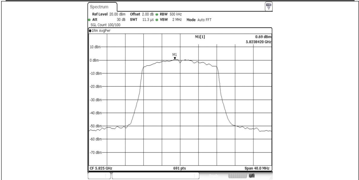
11A-Ant1-5825-PASS
