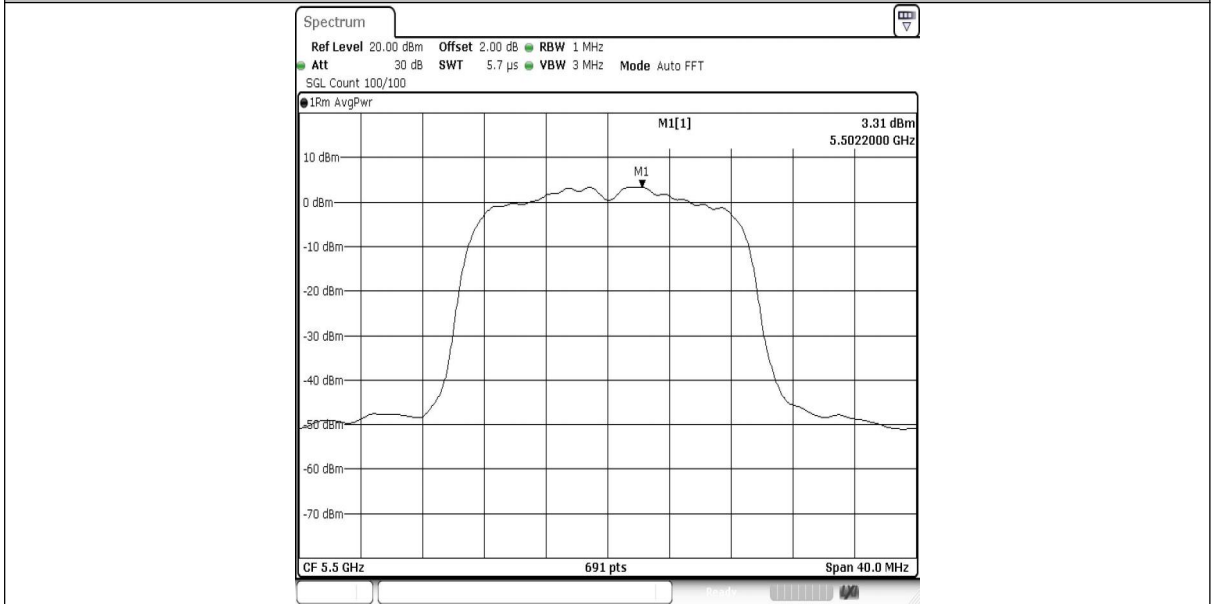
11N20SISO-Ant1-5500-PASS
