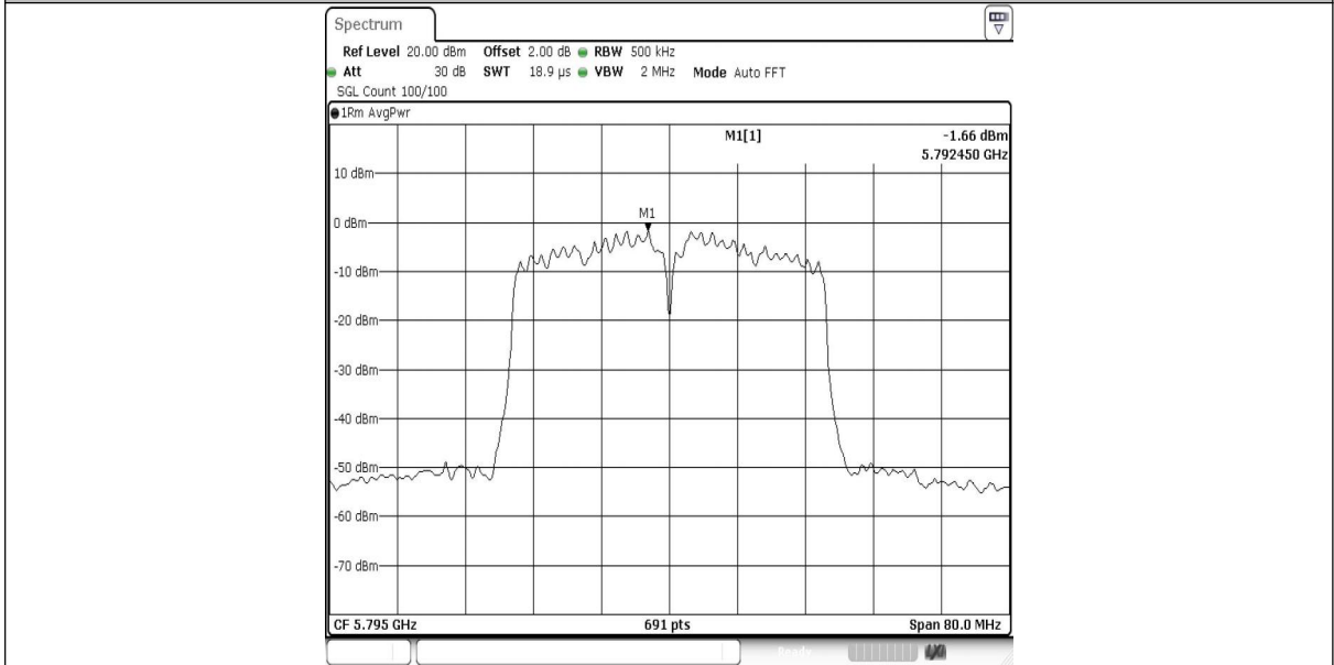
11N40SISO-Ant1-5795-PASS
