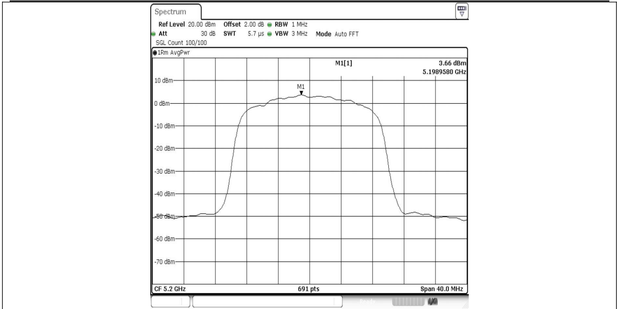
11N20SISO-Ant1-5200-PASS
