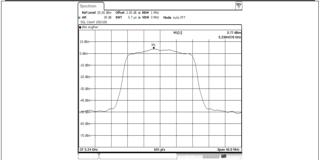
11A-Ant1-5240-PASS
