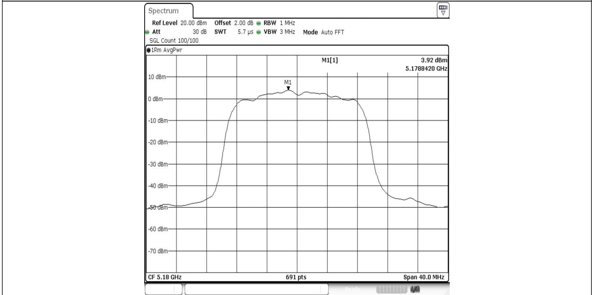
11N20SISO-Ant1-5180-PASS
