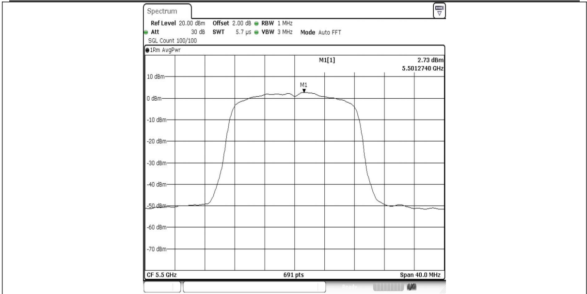
11A-Ant1-5500-PASS
