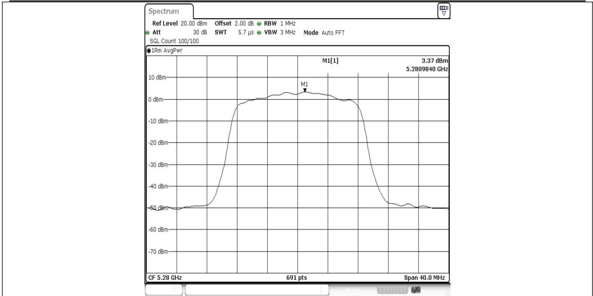
11A-Ant1-5280-PASS
