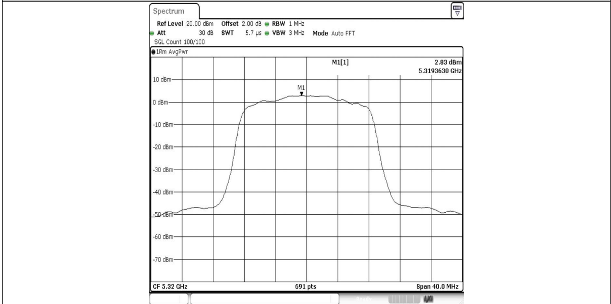
11A-Ant1-5320-PASS
