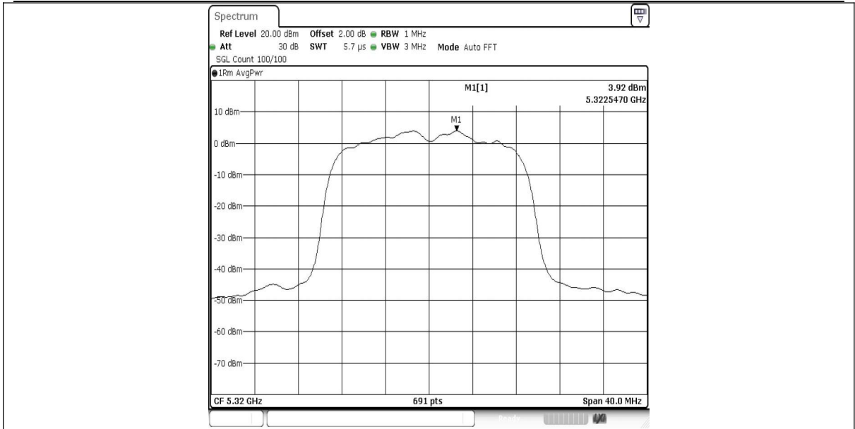
11N20SISO-Ant1-5320-PASS
