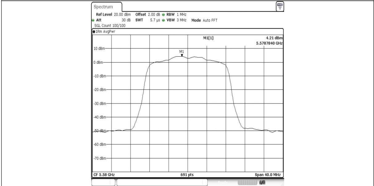
11A-Ant1-5580-PASS
