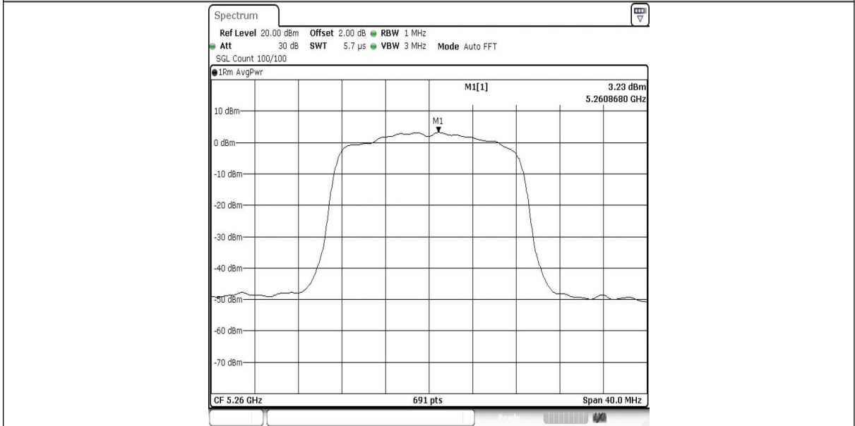
11A-Ant1-5260-PASS
