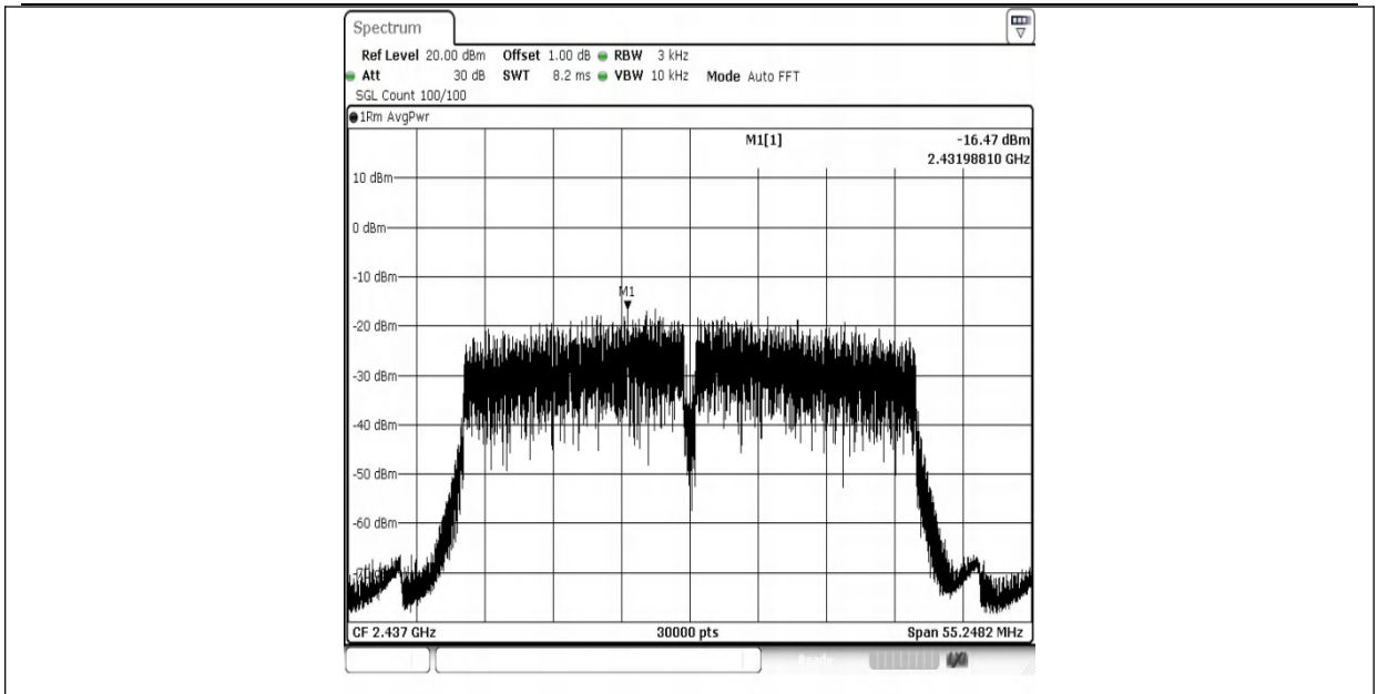
11N40SISO-Ant1-2437-PASS
