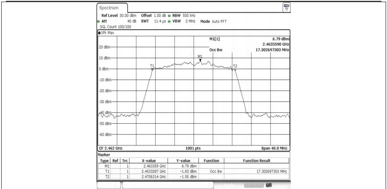
11N20SISO-Ant1-2462
