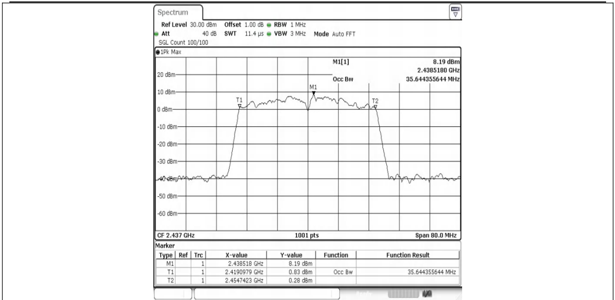
11N40SISO-Ant1-2437
