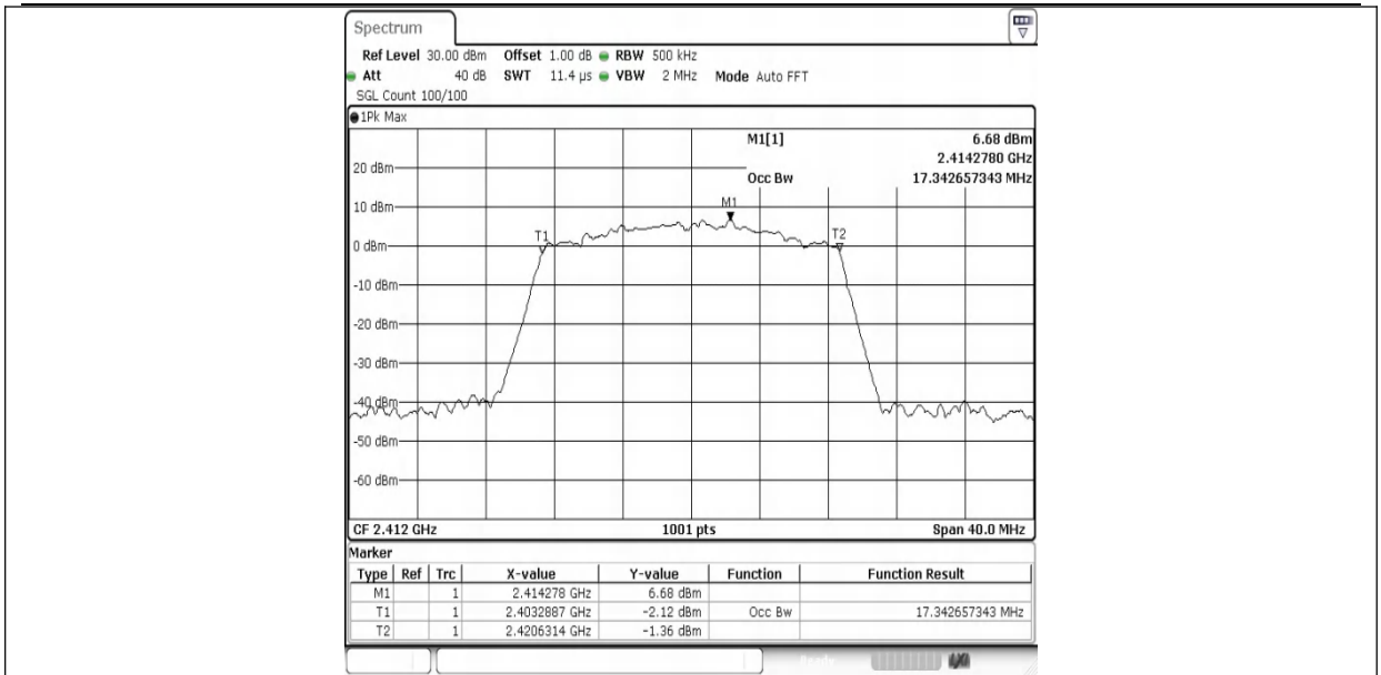
11N20SISO-Ant1-2412
