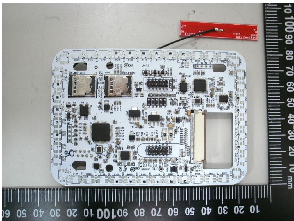
(ESP)+BT Board
