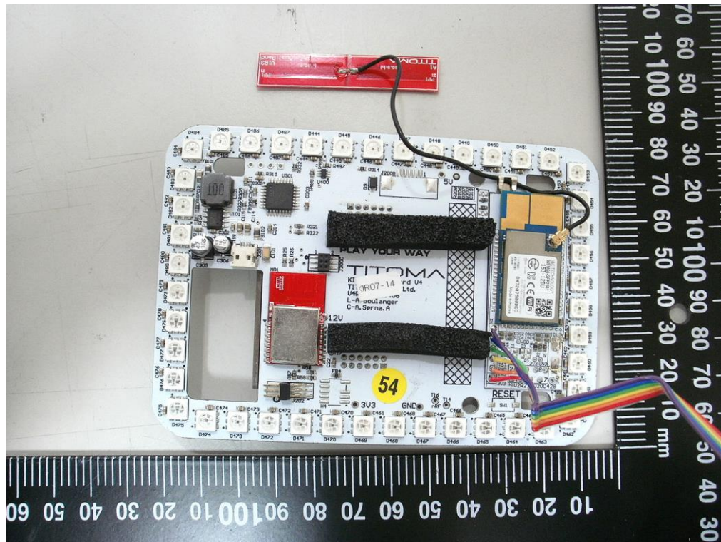
(WFM60)+BT Board
