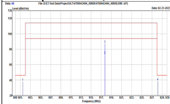
TX, Fundamental SRD Tx (Ch 12) Radiated Spurious Emission, Horizontal
