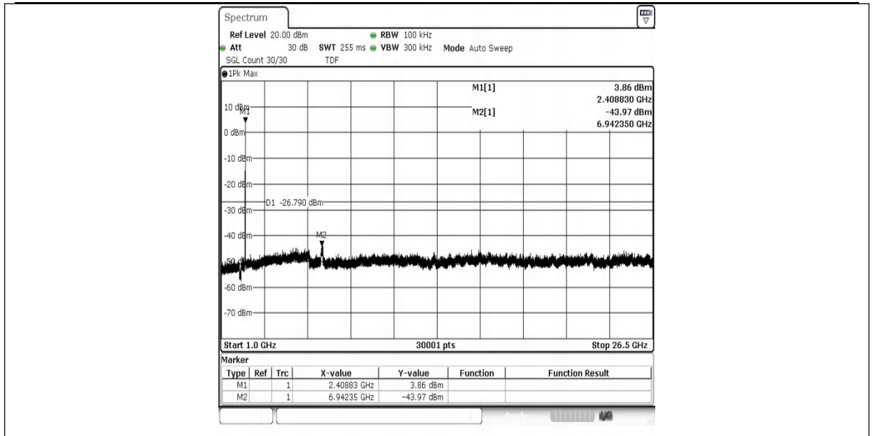
11B-Ant1-2412-1000~26500-PASS
