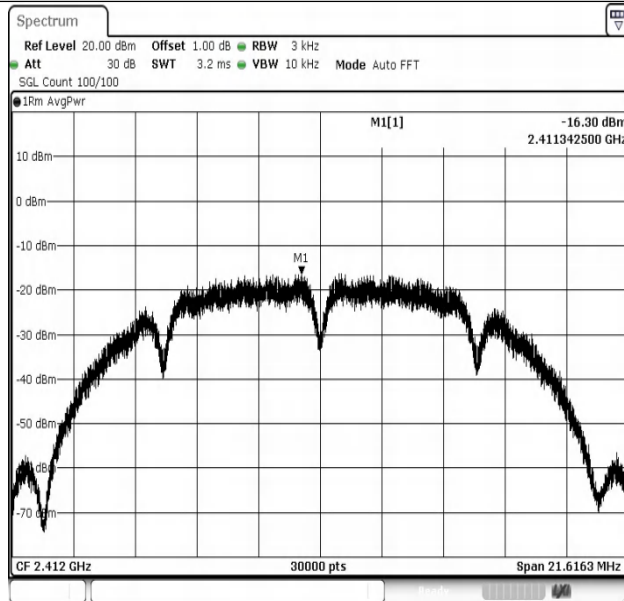
11B-Ant1-2412-PASS
