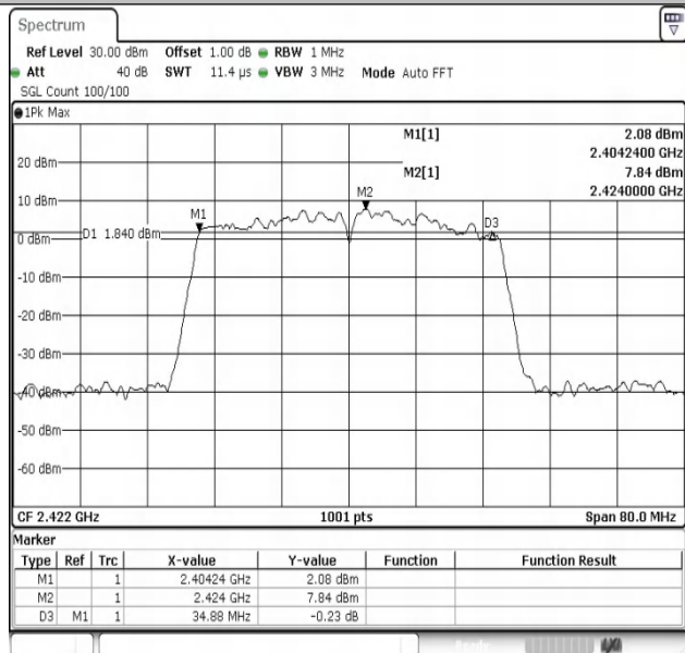
11N40SISO-Ant1-2422-PASS
