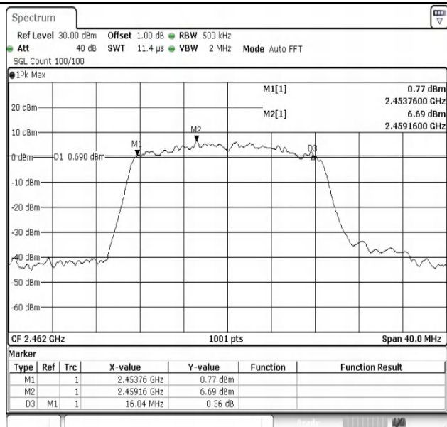
11N20SISO-Ant1-2462-PASS
