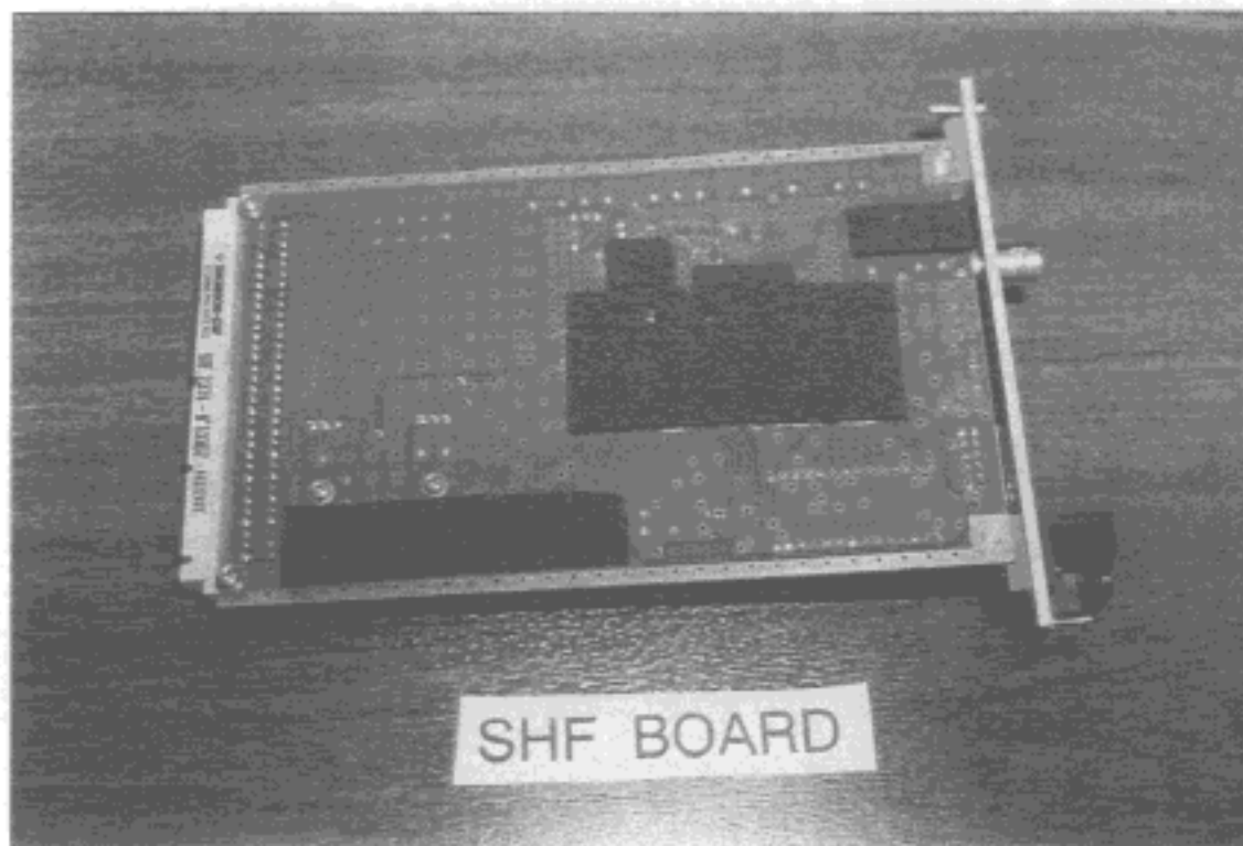
8-13 SHF foil side module and absorber location
