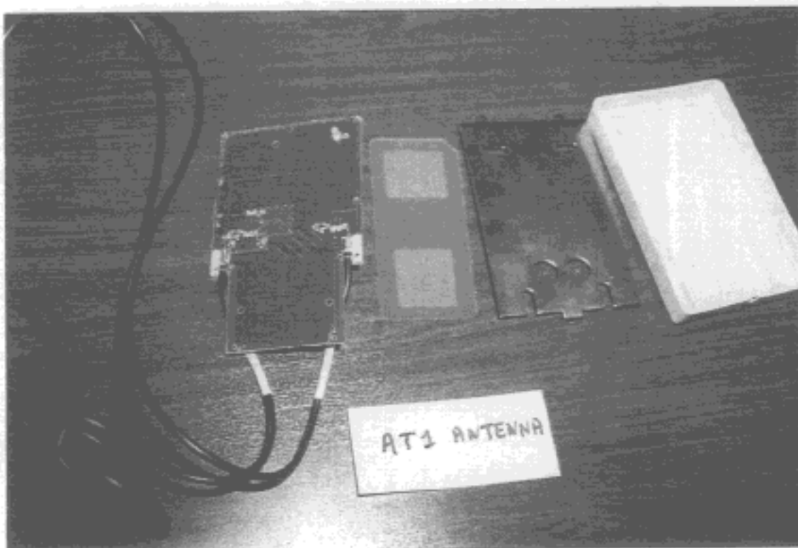
8-20 AT1 antenna inside (continued)
