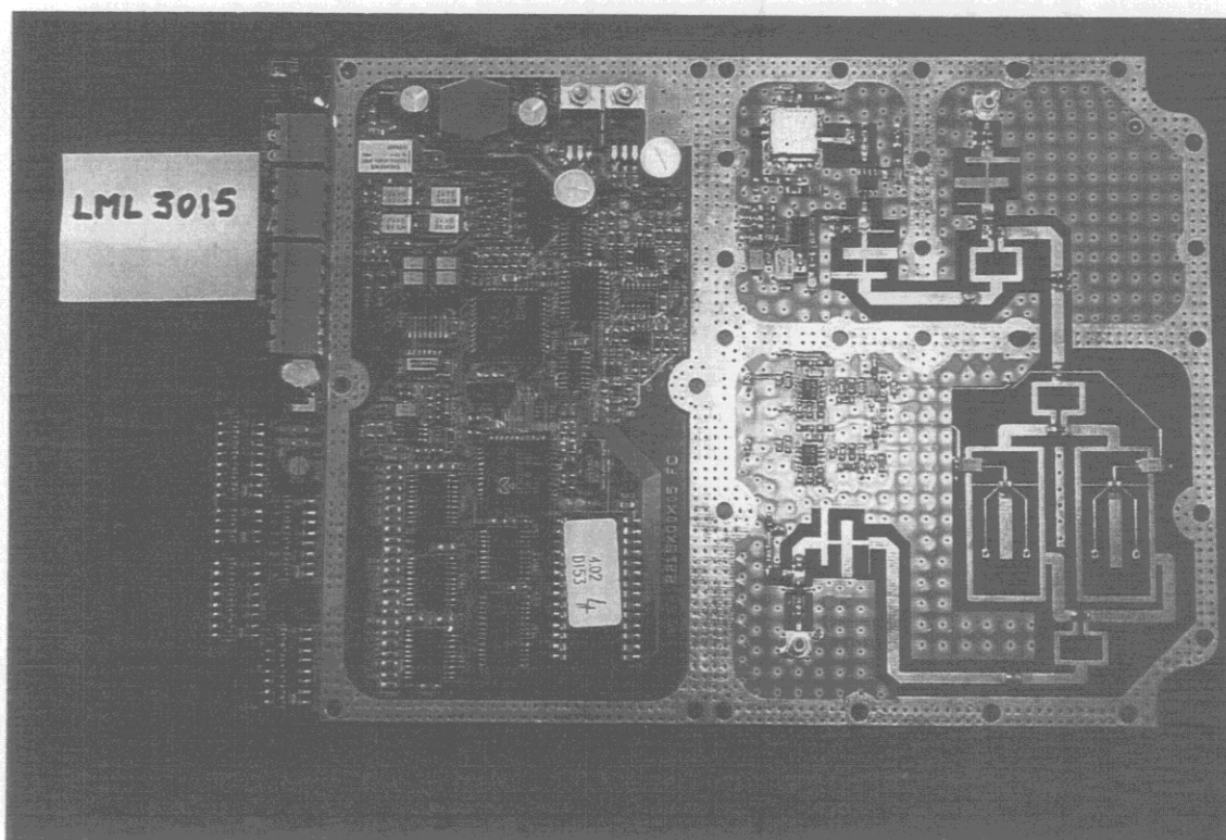
8-10 LML_3015 component side board
