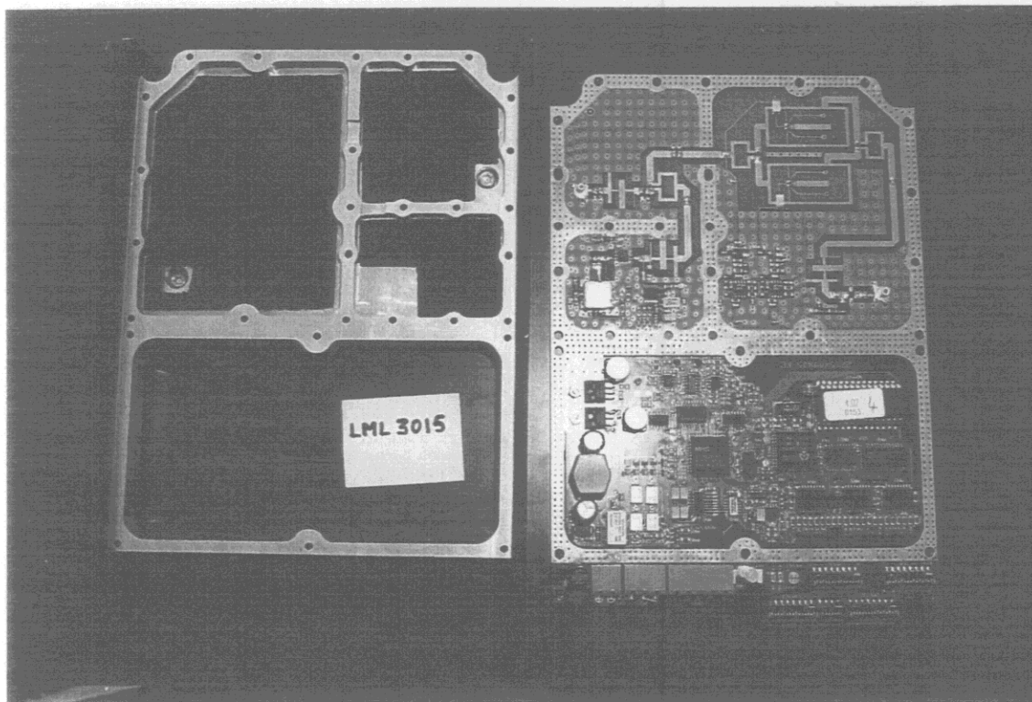
8-8 Inside reader LML_3015, metallic frame removed
