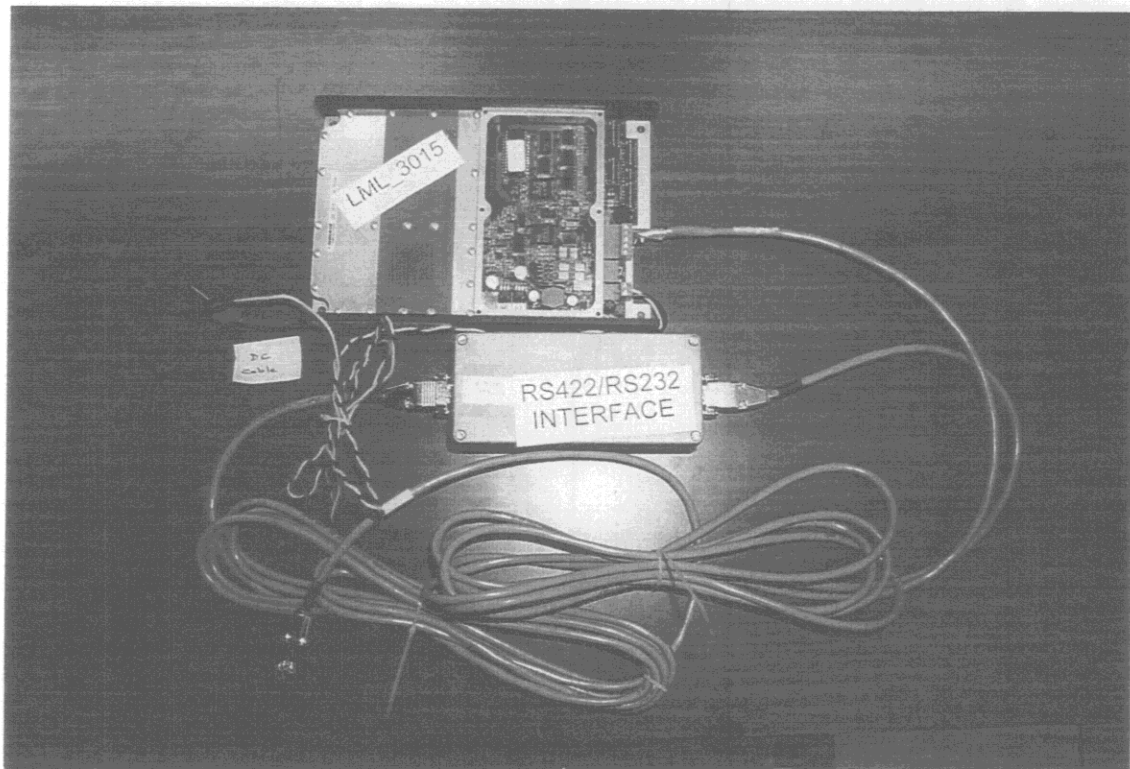
8-3 Reader LML_3015 with RS422 interface box and cables
