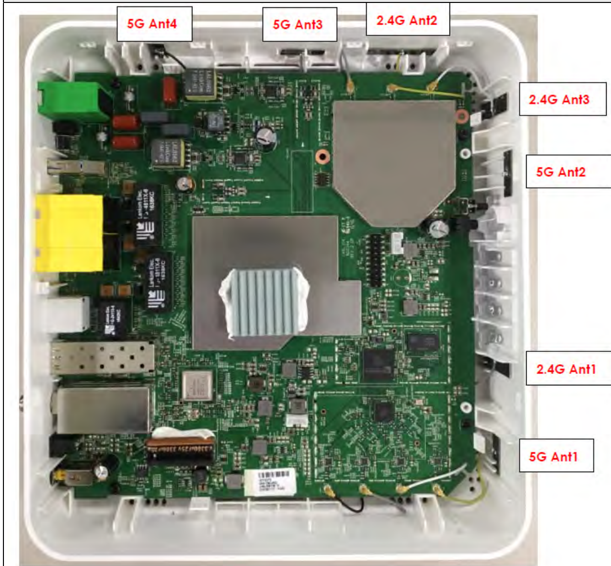
Antenna location
