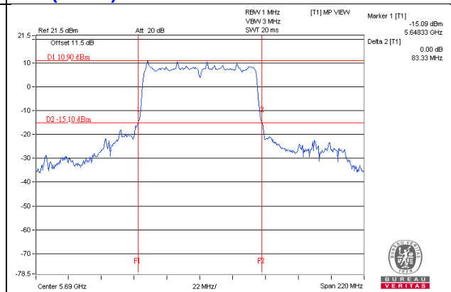
11ac (80MHz) 1S4T TXBF CH138 Chain4
