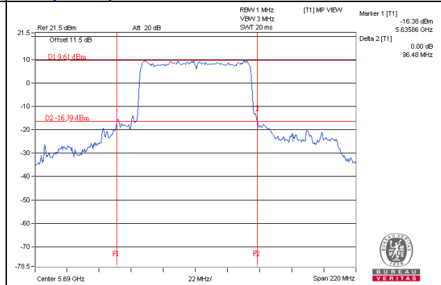
11ac (80MHz) 1S4T CDD CH138 Chain4
