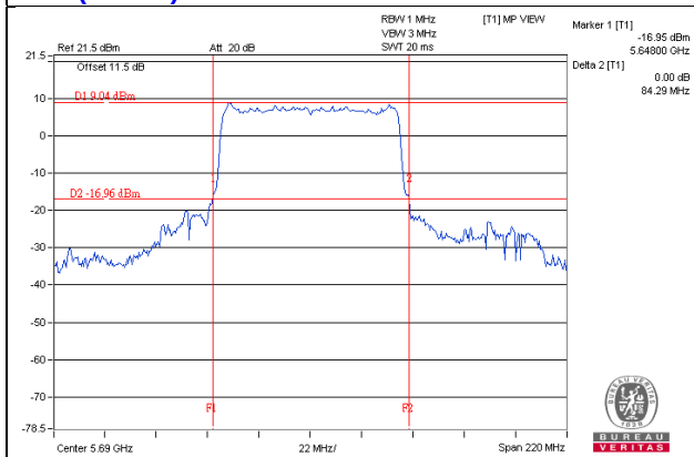
11ac (80MHz) 1S4T TXBF CH138 Chain3
