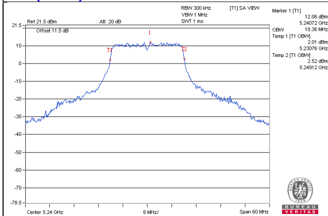
11ac (20MHz) 1S4T TXBF CH48 Chain1
