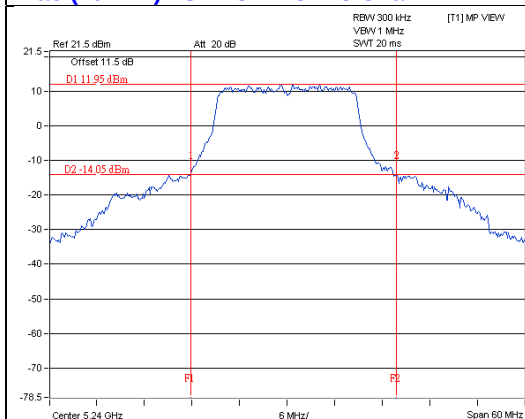
11ac (20MHz) 1S4T CDD CH48 Chain1
