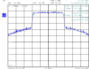
99 % Occupied Bandwidth
