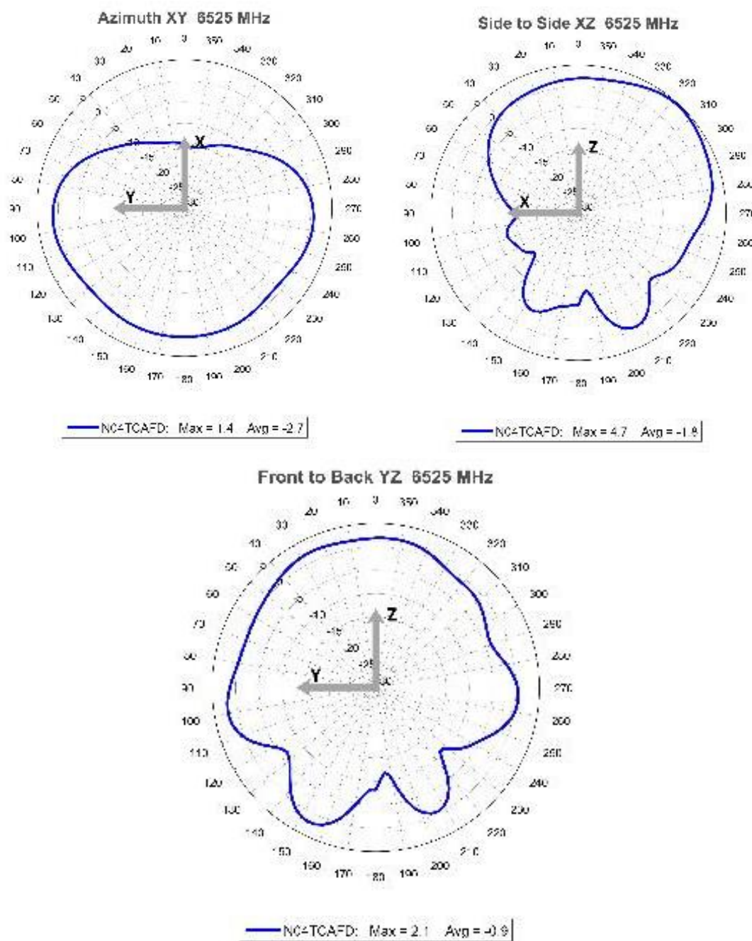
Figure 4: Model N04TCAFD Radiation Patterns at 6.525 GHz
