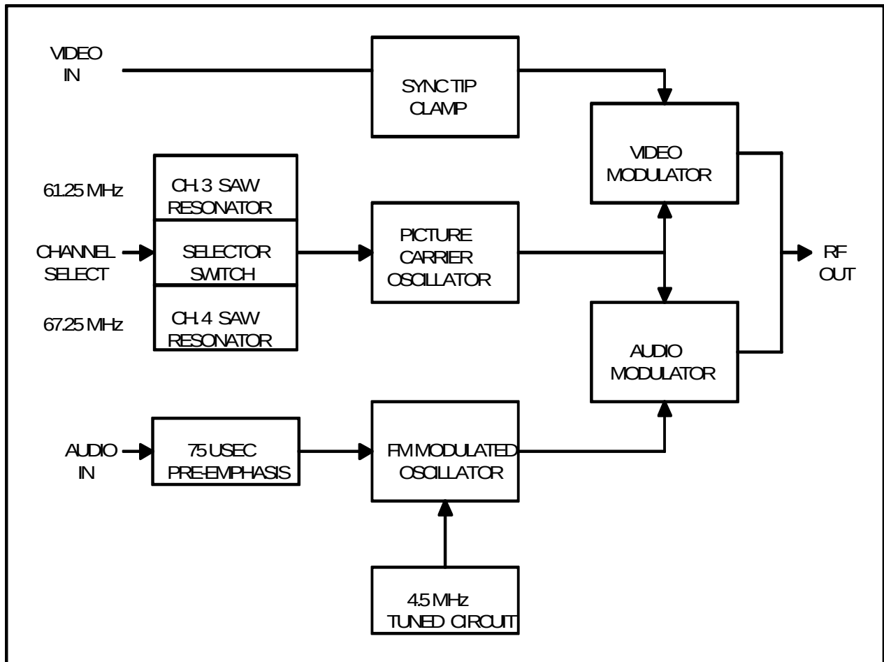
CH 3-4 MODULATOR
