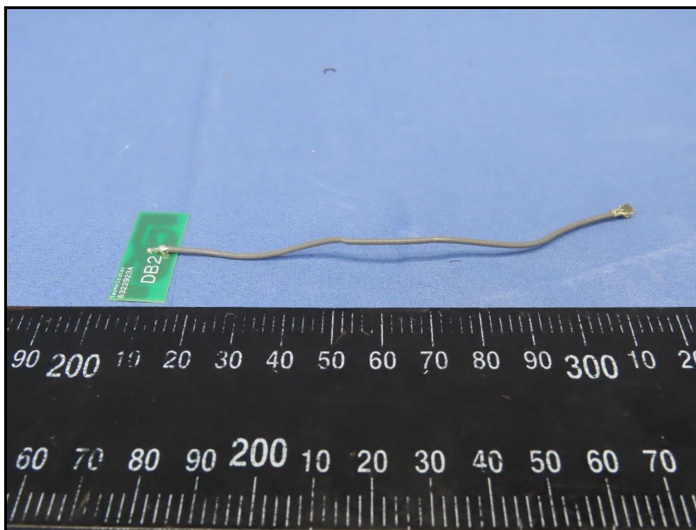
DB2 Antenna
