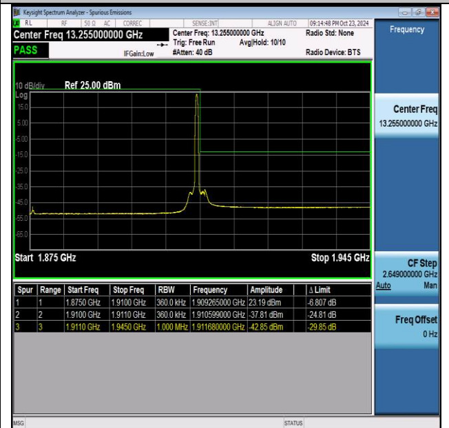
NTNV-n2-PC3-15-35-H-DFT-PI2BPSK-Edge_1RB_Right-PASS
