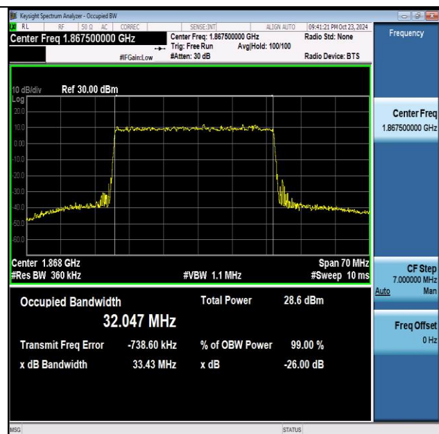
NTNV-n25-PC3-15-35-L-DFT-256QAM-Outer_Full-Ant1- PASS
