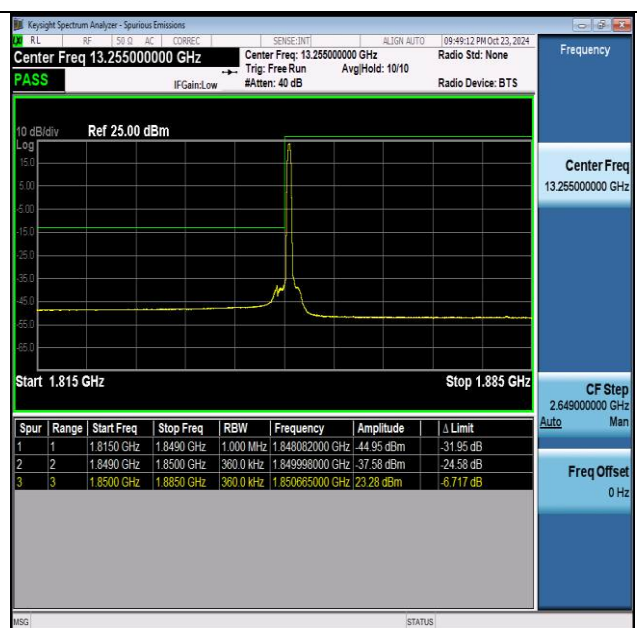
NTNV-n25-PC3-15-35-L-DFT-PI2BPSK-Edge_1RB_Left-PASS
