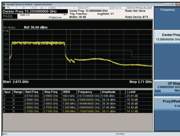
NTNV-n41-PC2-30-15-H-DFT-BPSK-Outer_Full-PASS
