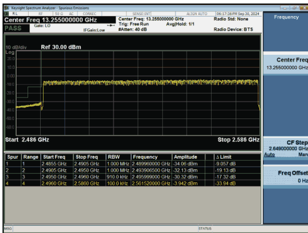
NTNV-n41-PC2-30-90-L-CP-QPSK-Outer_Full-PASS
