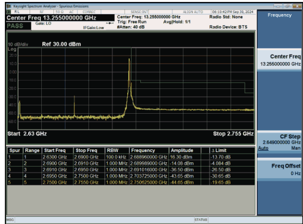
NTNV-n41-PC2-30-60-H-CP-QPSK-Edge_1RB_Right-PASS
