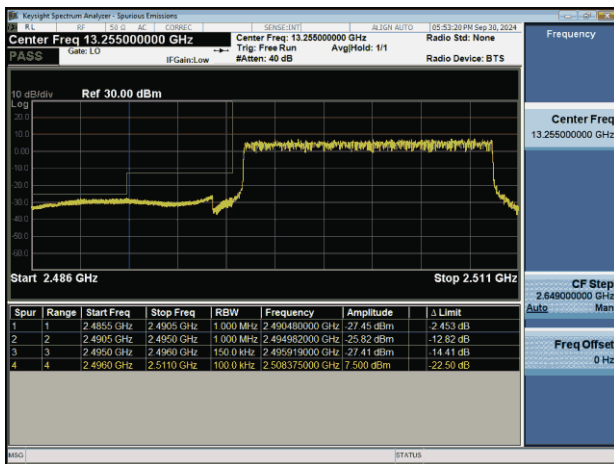
NTNV-n41-PC2-30-15-L-DFT-BPSK-Outet_Full-PASS
