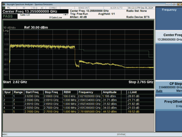
NTNV-n41-PC2-30-70-H-DFT-BPSK-Outter_Full-PASS
