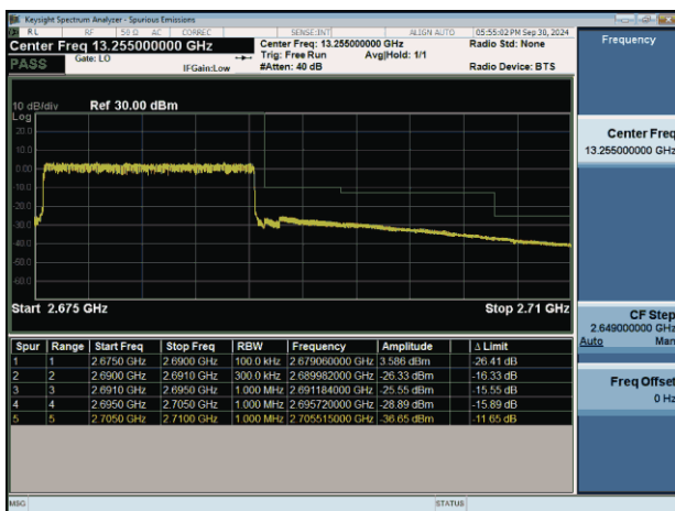
NTNV-n41-PC2-30-15-H-CP-QPSK-Outer_Full-PASS
