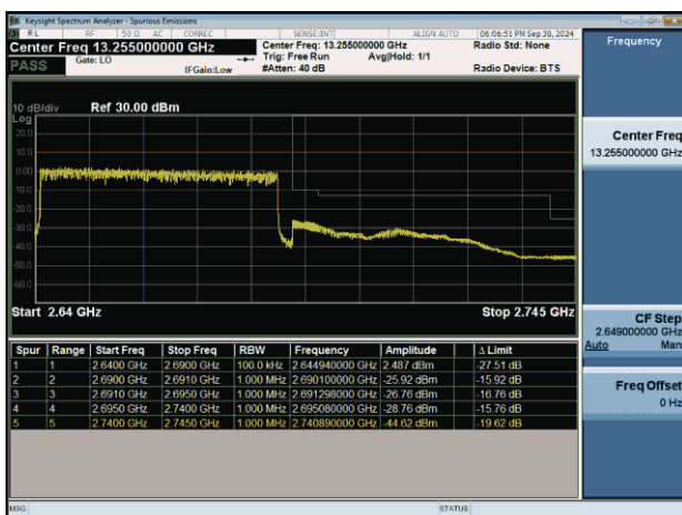
NTNV-n41-PC2-30-50-L-CP-QPSK-Outter_Full-PASS
