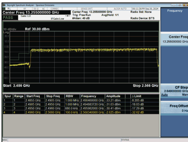
NTNV-n41-PC2-30-70-L-CP-QPSK-Outet_Full-PASS
