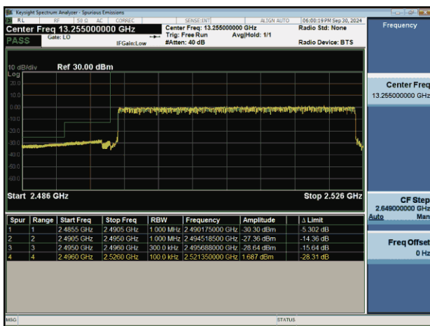
NTNV-n41-PC2-30-30-L-CP-QPSK-Outer_Full-PASS
