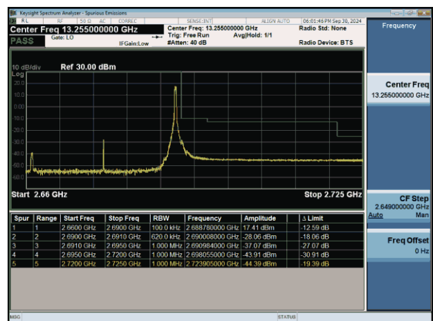
NTNV-n41-PC2-30-30-H-DFT-BPSK-Edge_1RB_Right-PASS
