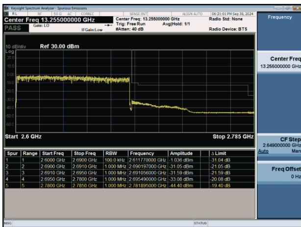
NTNV-n41-PC2-30-90-H-DFT-BPSK-Outer_Full-PASS
