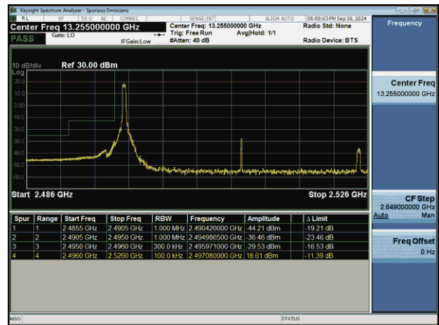
NTNV-n41-PC2-30-30-L-DFT-BPSK-Edge_1RB_Left-PASS
