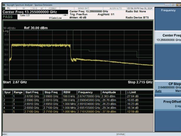
NTNV-n41-PC2-30-20-H-CP-QPSK-Outter_Full-PASS
