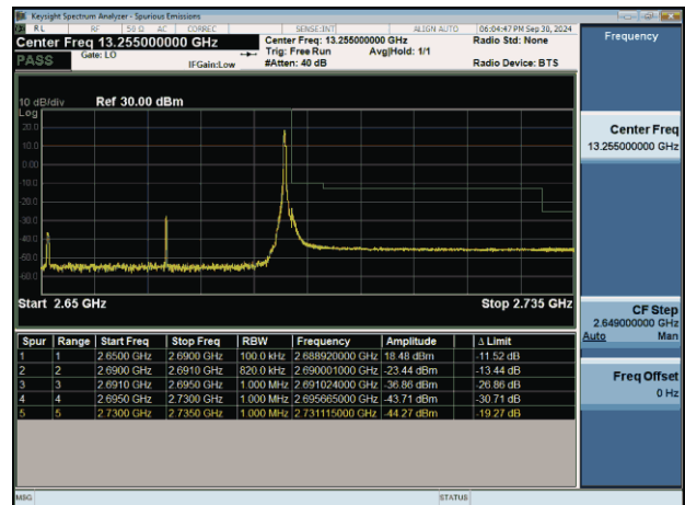
NTNV-n41-PC2-30-40-H-DFT-BPSK-Edge_1RB_Right-PASS
