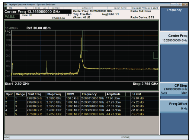
NTNV-n41-PC2-30-70-H-DFT-BPSK-Edge_1RB_Right-PASS
