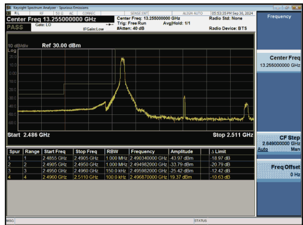
NTNV-n41-PC2-30-15-L-DFT-BPSK-Edge_1RB_Left-PASS
