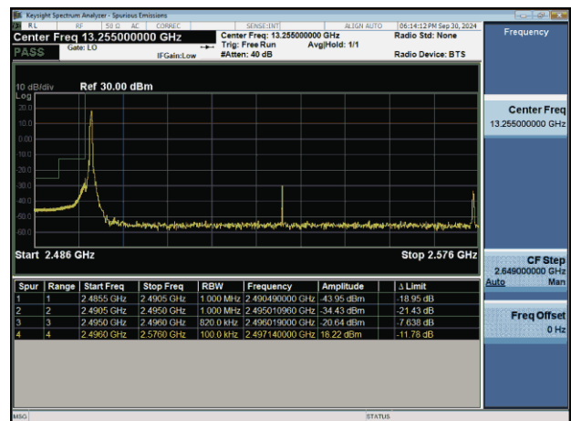
NTNV-n41-PC2-30-80-L-DFT-BPSK-Edge_1RB_Left-PASS
