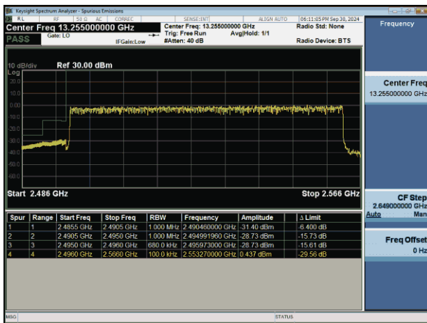
NTNV-n41-PC2-30-70-L-DFT-BPSK-Outet_Full-PASS
