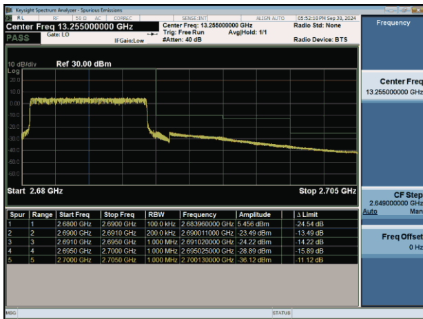
NTNV-n41-PC2-30-10-H-CP-QPSK-Outet_Full-PASS
