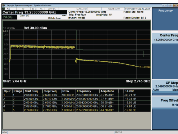
NTNV-n41-PC2-30-50-H-CP-QPSK-Outter_Full-PASS
