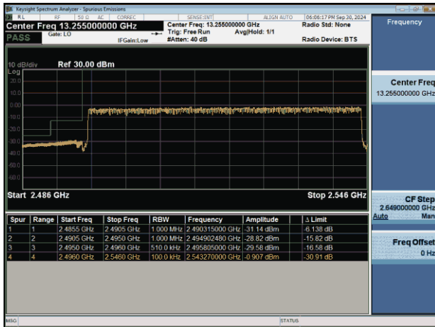
NTNV-n41-PC2-30-50-L-CP-QPSK-Outter_Full-PASS
