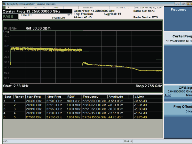
NTNV-n41-PC2-30-60-H-CP-QPSK-Outet_Full-PASS
