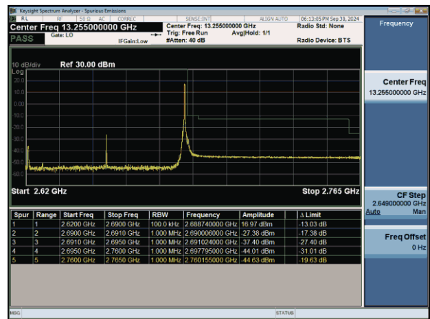
NTNV-n41-PC2-30-70-H-CP-QPSK-Edge_1RB_Right-PASS
