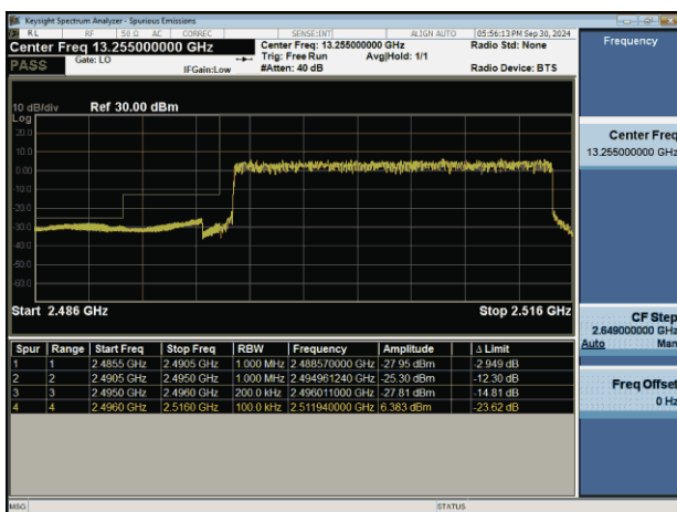
NTNV-n41-PC2-30-20-L-DFT-BPSK-Outer_Full-PASS
