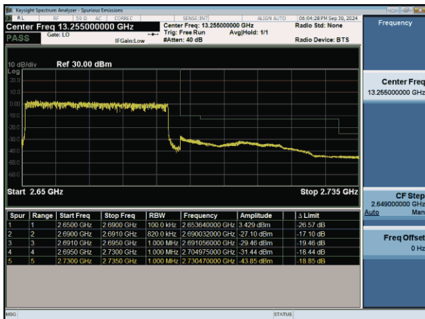
NTNV-n41-PC2-30-40-H-DFT-BPSK-Outer_Full-PASS
