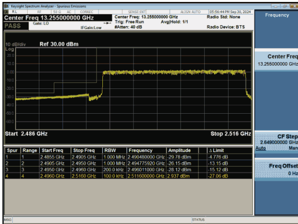
NTNV-n41-PC2-30-20-L-CP-QPSK-Outter_Full-PASS
