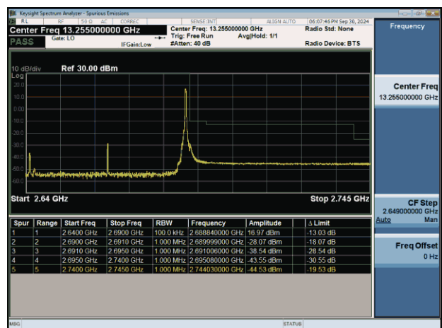
NTNV-n41-PC2-30-50-H-CP-QPSK-Edge_1RB_Right-PASS
