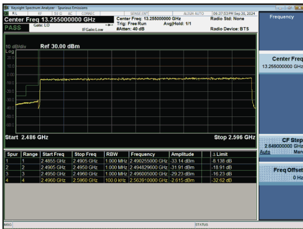
NTNV-n41-PC2-30-100-L-DFT-BPSK-Outer_Full-PASS
