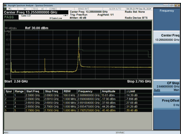
NTNV-n41-PC2-30-100-H-CP-QPSK-Edge_1RB_Right-PASS
