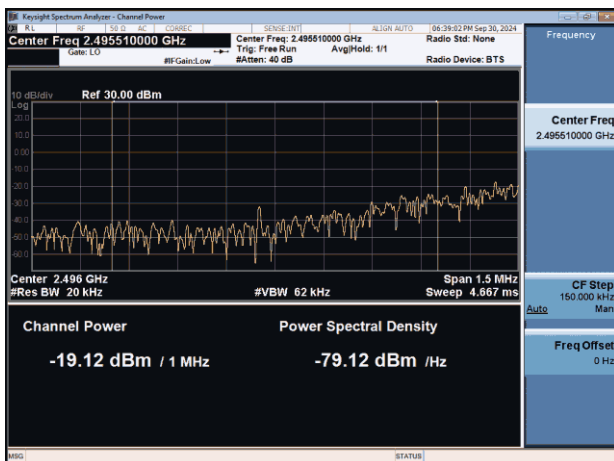
NTNV-n41-PC2-30-100-L-DFT-BPSK-Edge_1RB_Left-PASS
