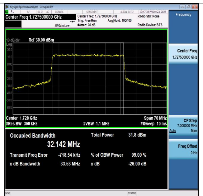
NTNV-n66-PC3-15-35-L-DFT-QPSK-Outter_Full-Ant1- PASS
