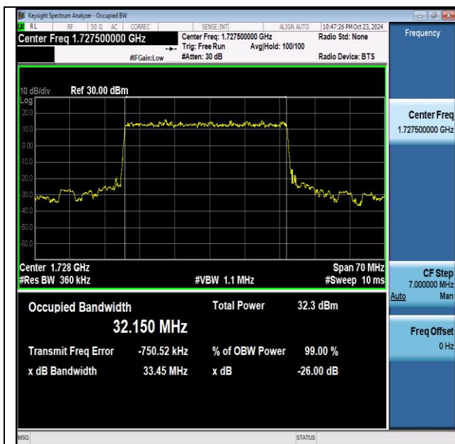
NTNV-n66-PC3-15-35-L-DFT-BPSK-Outter_Full-Ant1- PASS
