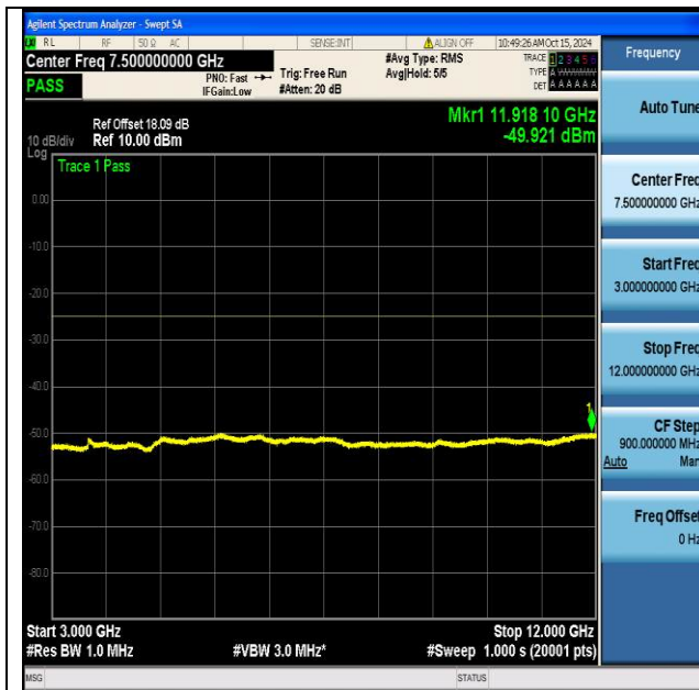
NTNV_N7_PC3_15_40_L_TID1_NS_01_3000_12000_#1
