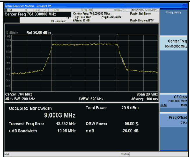
Band12-10MHz-256QAM-23060-50RB#0-PASS
