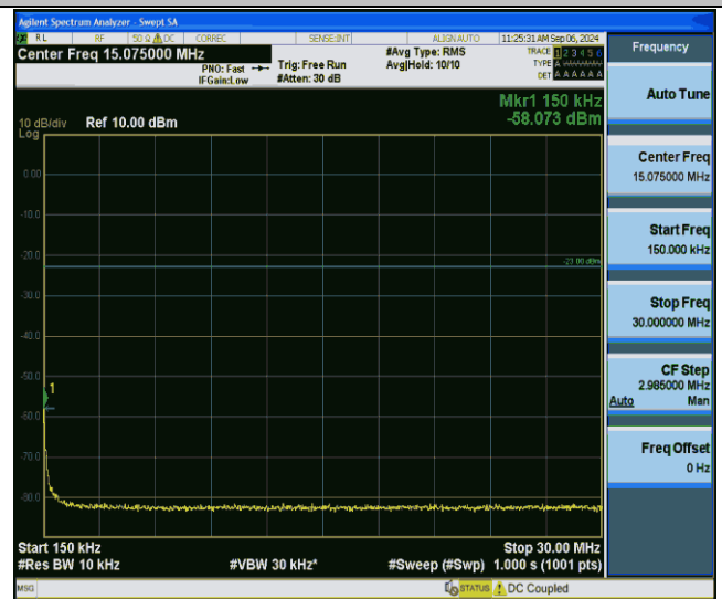
Band12-10MHz-QPSK-23130-1RB#0-0.15~30-PASS
