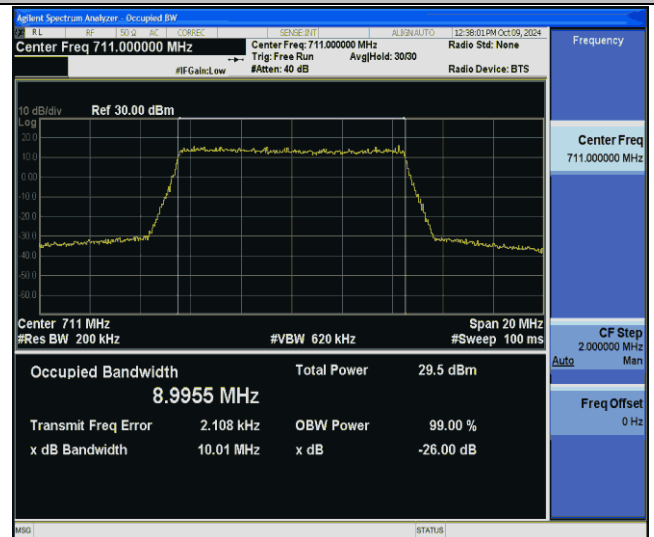
Band12-10MHz-256QAM-23130-50RB#0-PASS
