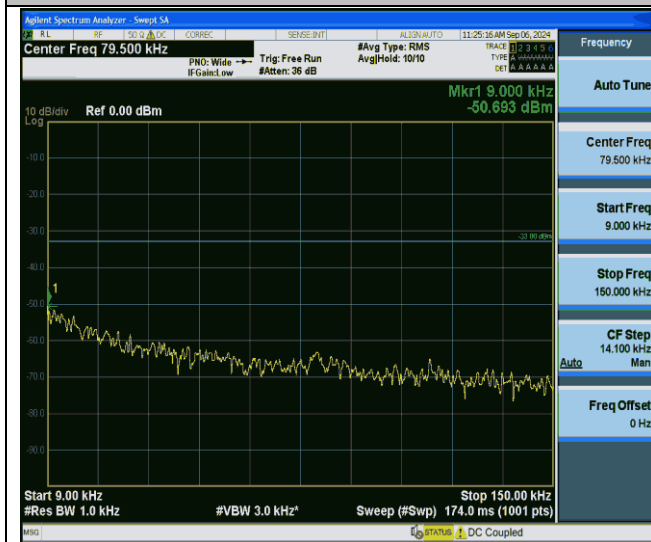
Band12-10MHz-QPSK-23130-1RB#0-0.009~0.15-PASS
