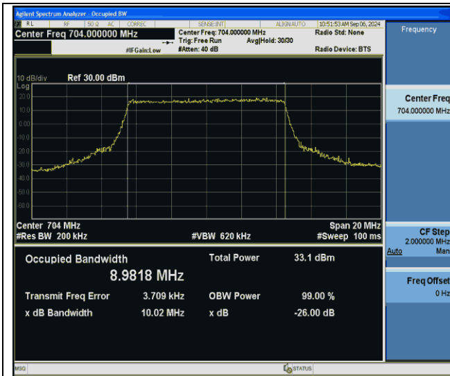
Band12-10MHz-QPSK-23060-50RB#0-PASS
