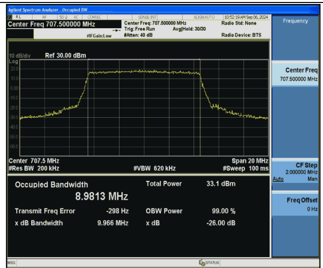
Band12-10MHz-QPSK-23095-50RB#0-PASS
