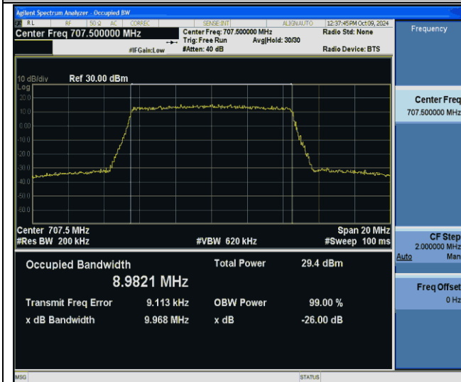
Band12-10MHz-256QAM-23095-50RB#0-PASS
