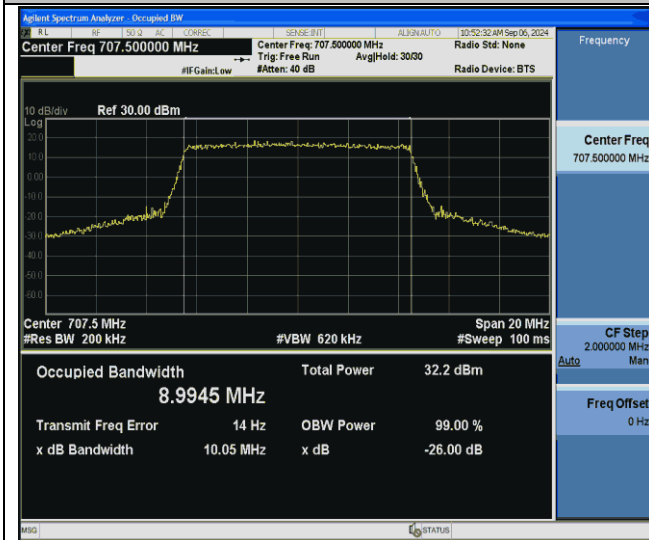
Band12-10MHz-16QAM-23095-50RB#0-PASS
