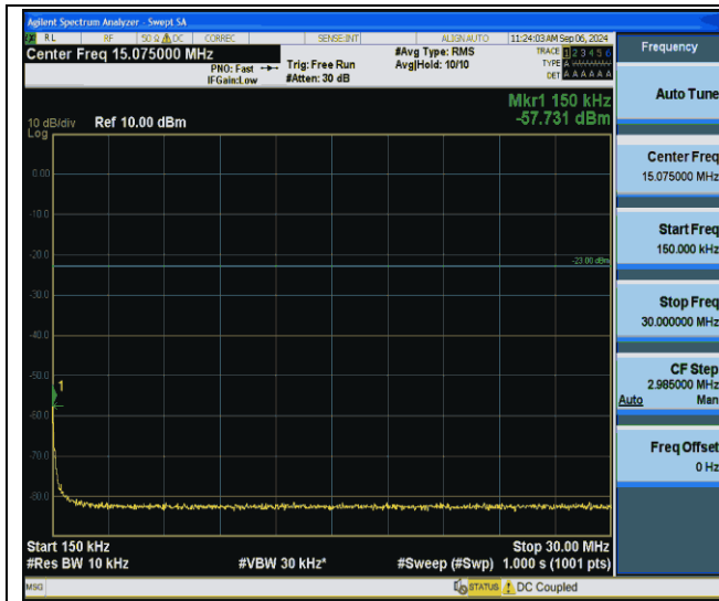
Band12-10MHz-QPSK-23095-1RB#0-0.15~30-PASS
