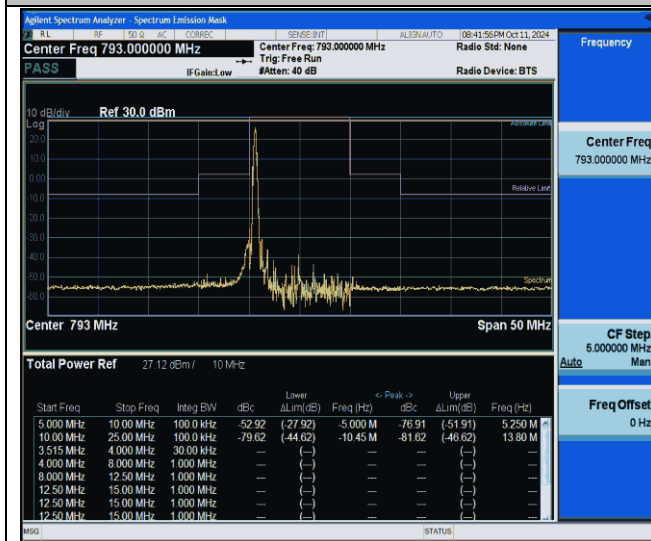
NTVN-Band14-10MHz-QPSK-23330-1RB#0-5.00-10.00-PASS
