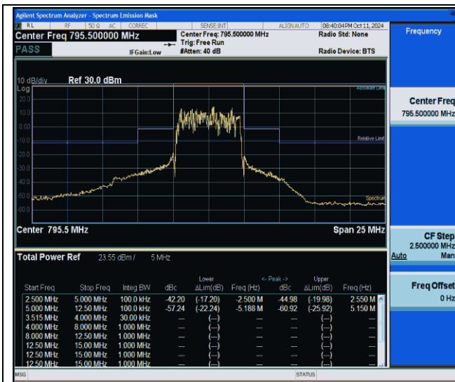
NTNV-Band14-5MHz-QPSK-23355-25RB#0--5.00--2.50-PASS
