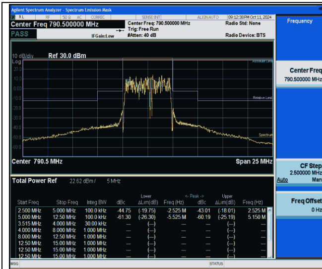
NTNV-Band14-5MHz-64QAM-23305-25RB#0--5.00--2.50-PASS
