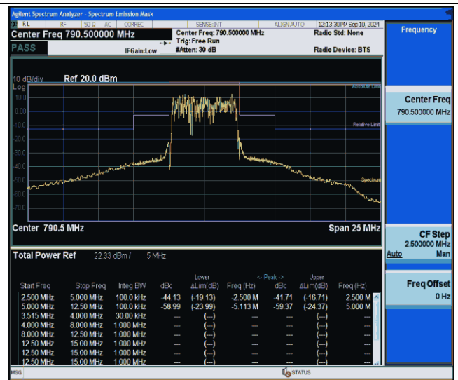
NTNV-Band14-5MHz-64QAM-23305-25RB#0--2.50-2.50-PASS
