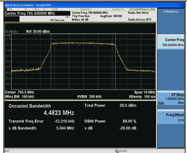
Band14-5MHz-256QAM-23355-25RB#0-PASS
