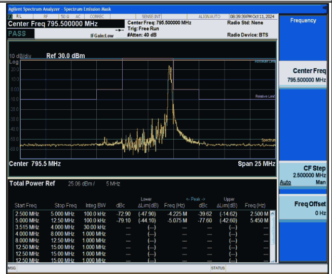
NTNV-Band14-5MHz-QPSK-23355-1RB#24--2.50-2.50-PASS
