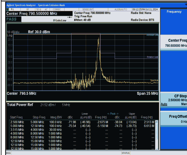
NTNV-Band14-5MHz-64QAM-23305-1RB#24--12.50--5.00-PASS
