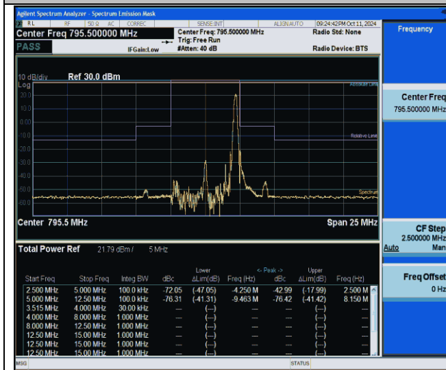
NTNV-Band14-5MHz-256QAM-23355-1RB#24--12.50--5.00-PASS
