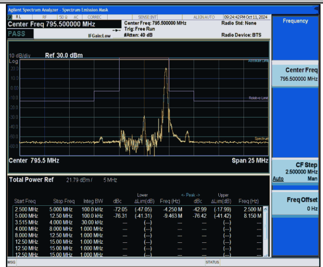
NTNV-Band14-5MHz-256QAM-23355-1RB#24--5.00--2.50-PASS
