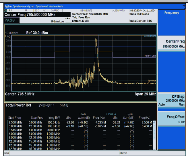
NTNV-Band14-5MHz-QPSK-23355-1RB#24--12.50--5.00-PASS
