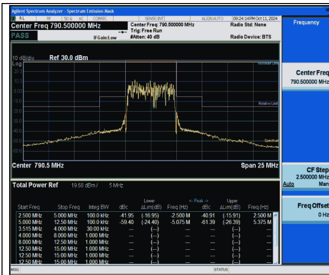
NTNV-Band14-5MHz-256QAM-23305-25RB#0--2.50-2.50-PASS
