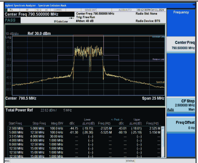
NTNV-Band14-5MHz-64QAM-23305-25RB#0--12.50--5.00-PASS
