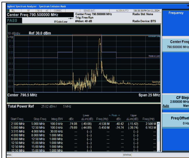
NTNV-Band14-5MHz-16QAM-23305-1RB#24-5.00-12.50-PASS
