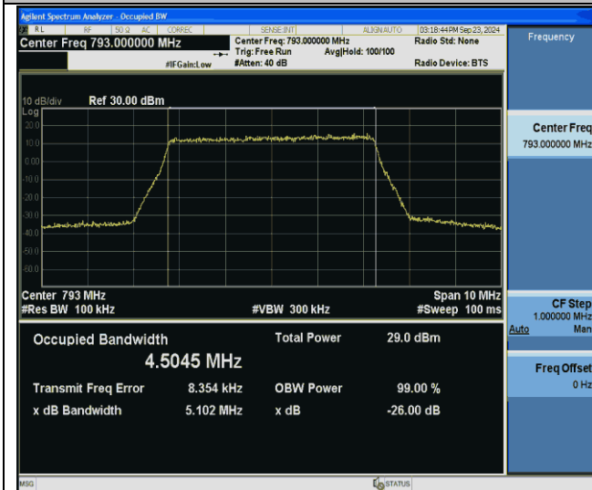
Band14-5MHz-256QAM-23330-25RB#0-PASS
