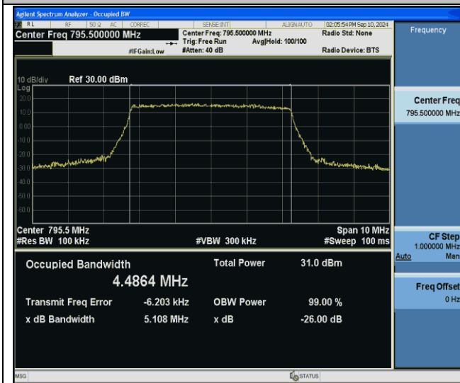
Band14-5MHz-64QAM-23355-25RB#0-PASS
