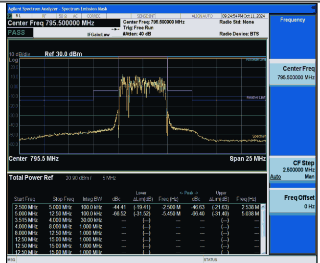
NTNV-Band14-5MHz-256QAM-23355-25RB#0--5.00--2.50-PASS
