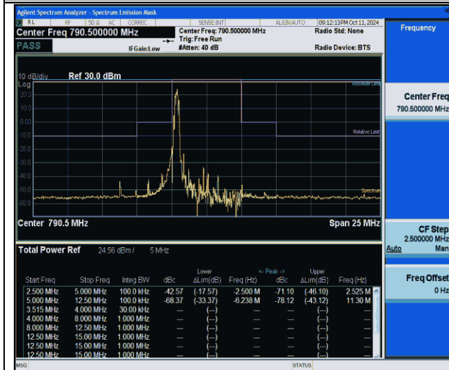
NTNV-Band14-5MHz-64QAM-23305-1RB#0-5.00-12.50-PASS
