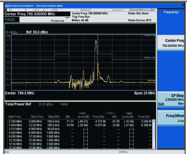
NTNV-Band14-5MHz-256QAM-23305-1RB#24-5.00-12.50-PASS
