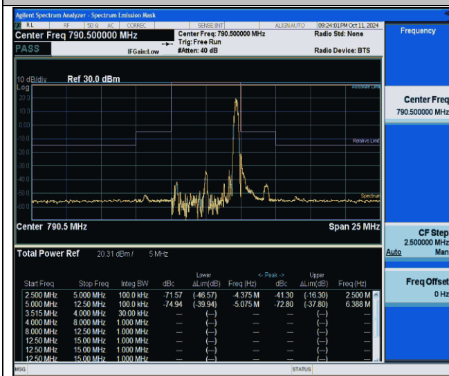
NTNV-Band14-5MHz-256QAM-23305-1RB#24--12.50--5.00-PASS
