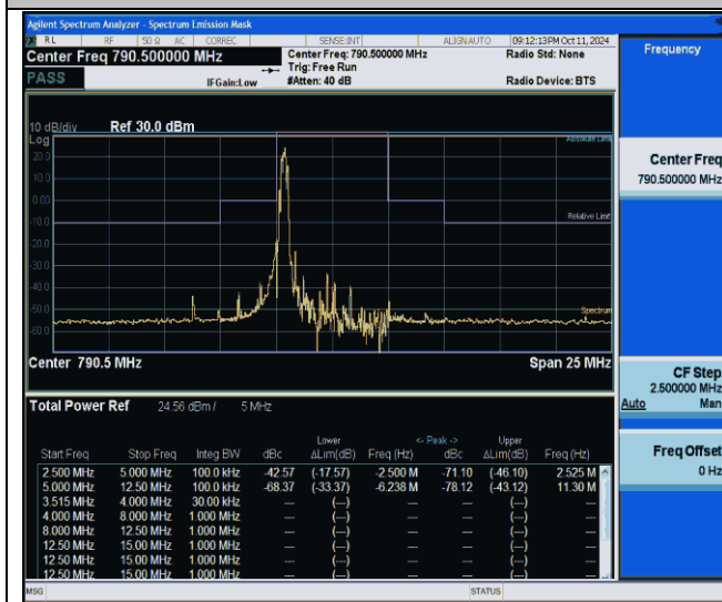
NTNV-Band14-5MHz-64QAM-23305-1RB#0--5.00--2.50-PASS
