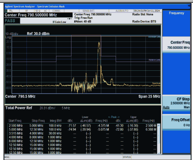
NTNV-Band14-5MHz-256QAM-23305-1RB#24--5.00--2.50-PASS
