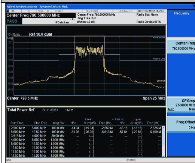
NTNV-Band14-5MHz-QPSK-23305-25RB#0-5.00-12.50-PASS
