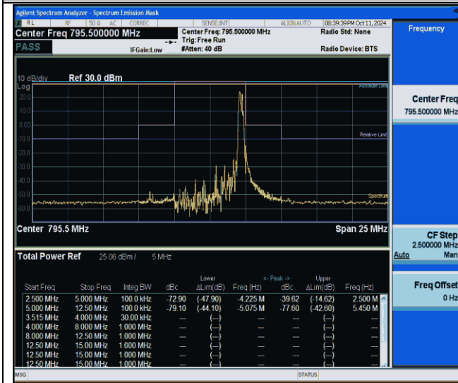
NTNV-Band14-5MHz-QPSK-23355-1RB#24--5.00--2.50-PASS
