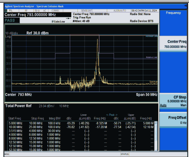
NTNV-Band14-10MHz-16QAM-23330-1RB#49--25.00--10.00-PASS
