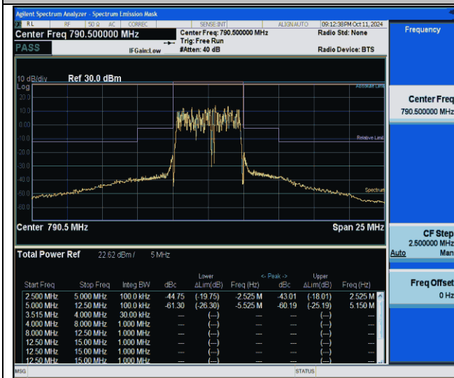
NTNV-Band14-5MHz-64QAM-23305-25RB#0-2.50-5.00-PASS
