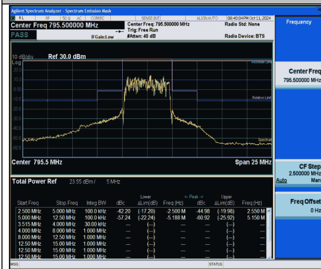
NTNV-Band14-5MHz-QPSK-23355-25RB#0-5.00-12.50-PASS
