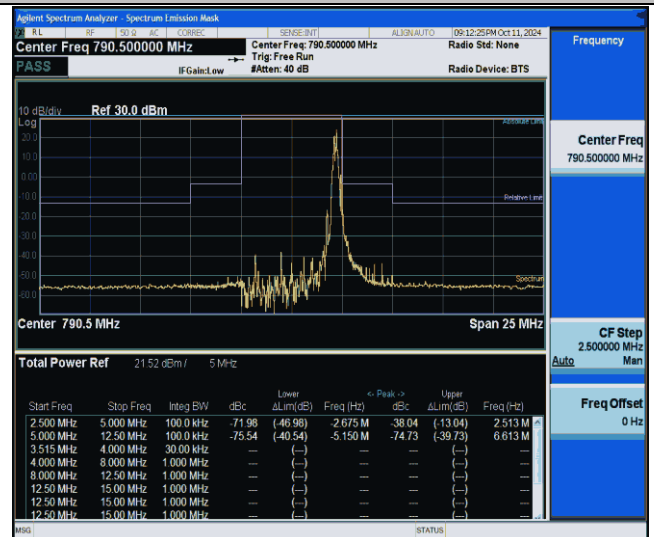
NTNV-Band14-5MHz-64QAM-23305-1RB#24--5.00--2.50-PASS
