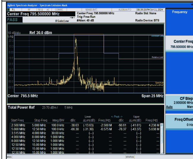
NTNV-Band14-5MHz-16QAM-23355-1RB#0-5.00-12.50-PASS
