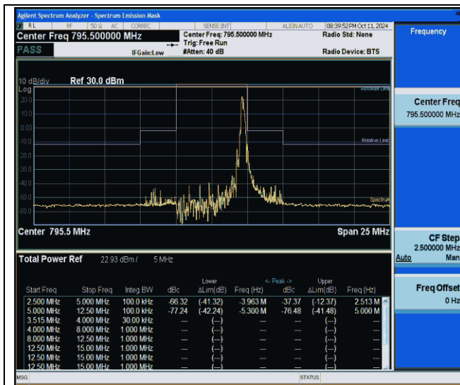
NTNV-Band14-5MHz-16QAM-23355-1RB#24-2.50-5.00-PASS
