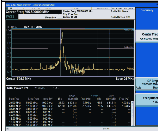
NTNV-Band14-5MHz-16QAM-23355-1RB#0--5.00--2.50-PASS
