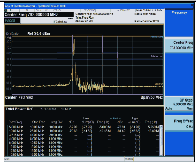
NTVN-Band14-10MHz-QPSK-23330-1RB#0-10.00-25.00-PASS
