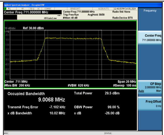
Band17-10MHz-256QAM-23800-50RB#0-PASS
