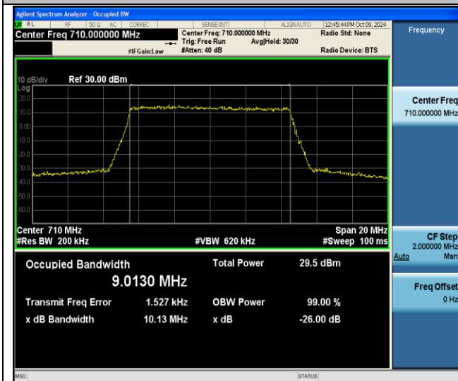
Band17-10MHz-256QAM-23790-50RB#0-PASS
