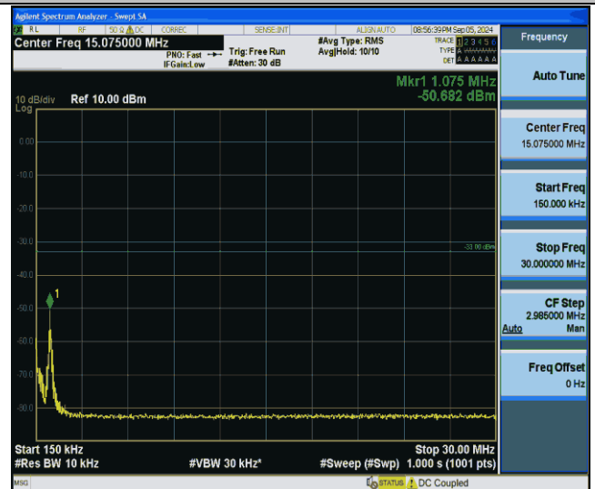
Band2-20MHz-QPSK-19100-1RB#0-0.15~30-PASS
