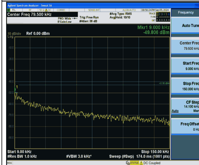
Band2-20MHz-QPSK-19100-1RB#0-0.009~0.15-PASS
