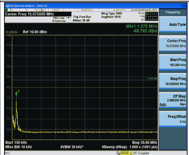
Band25-20MHz-QPSK-26590-1RB#0-0.15~30-PASS
