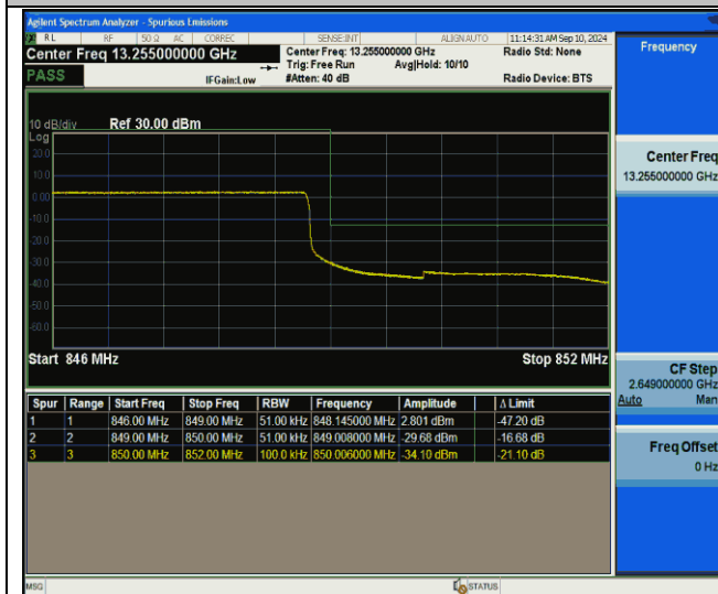
Band26(824-849)-5MHz-QPSK-27015-25RB#0-PASS
