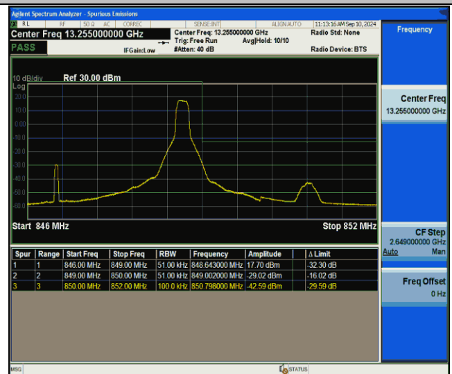
Band26(824-849)-5MHz-QPSK-27015-1RB#24-PASS
