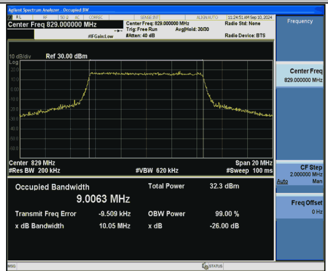
Band26(824-849)-10MHz-16QAM-26840-50RB#0-PASS
