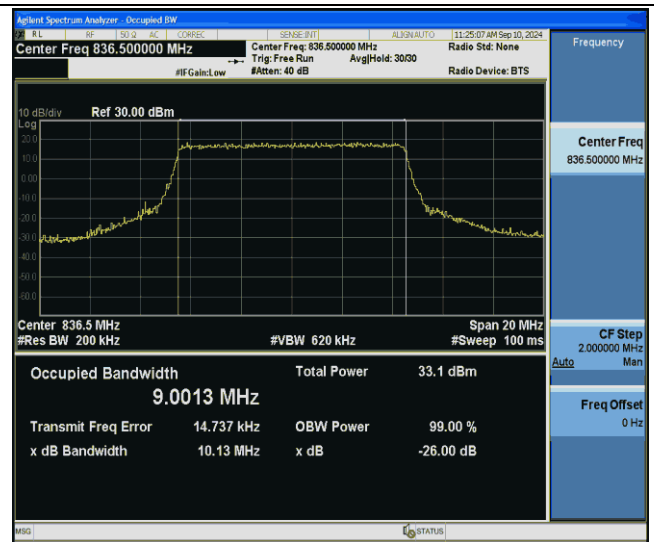
Band26(824-849)-10MHz-QPSK-26915-50RB#0-PASS
