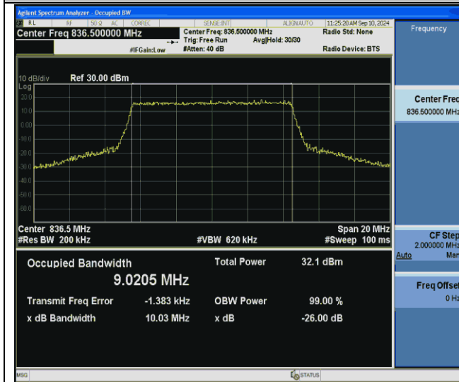
Band26(824-849)-10MHz-16QAM-26915-50RB#0-PASS
