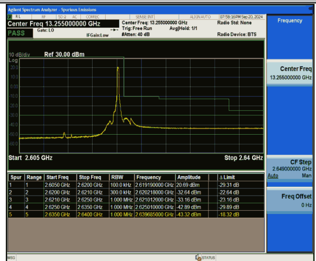
Band38-15MHz-QPSK-38175-1RB#74-PASS
