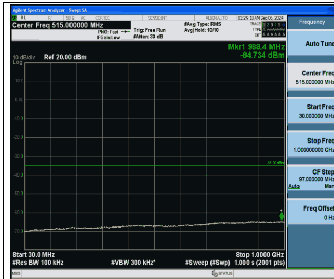
Band38-20MHz-QPSK-38150-1RB#0-30~1000-PASS
