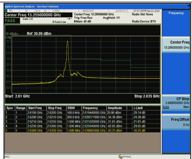
Band38-10MHz-QPSK-38200-1RB#49-PASS
