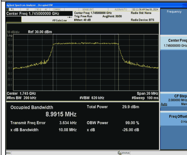
Band66-10MHz-16QAM-132322-50RB#0-PASS
