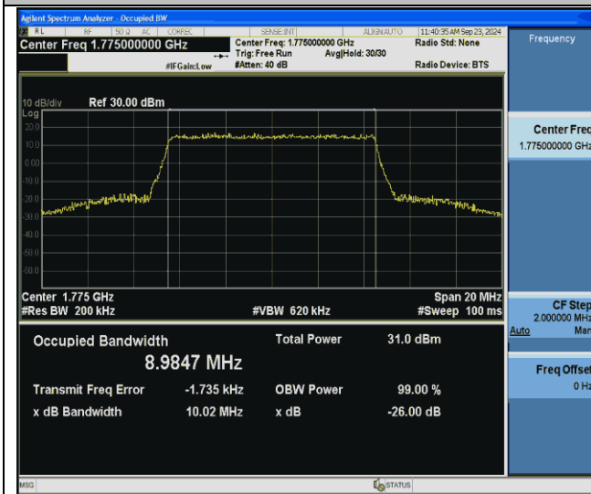
Band66-10MHz-64QAM-132622-50RB#0-PASS
