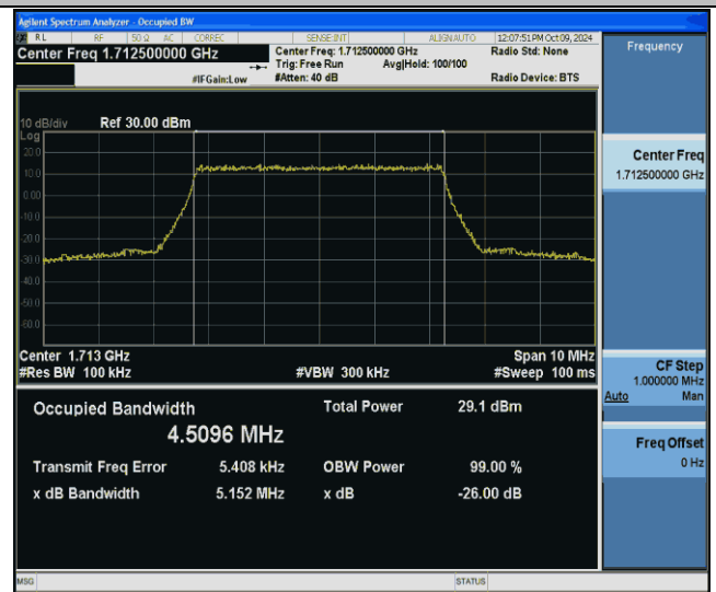
Band66-5MHz-256QAM-131997-25RB#0-PASS
