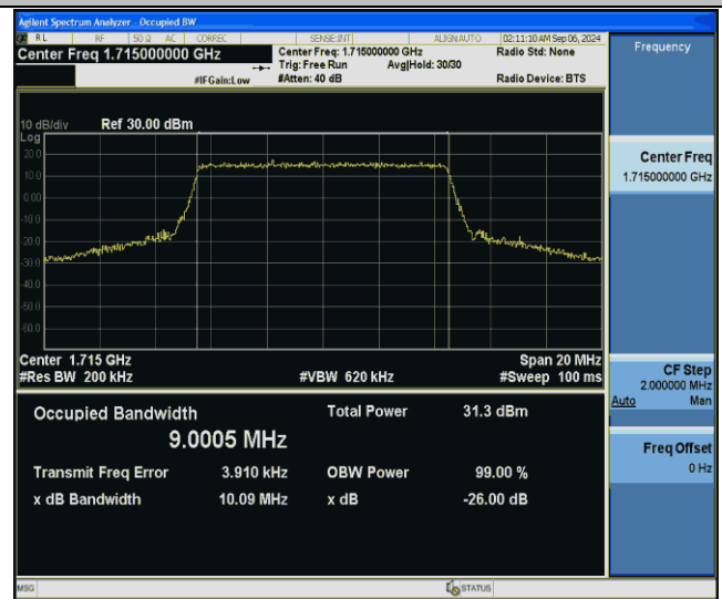
Band66-10MHz-16QAM-132022-50RB#0-PASS
