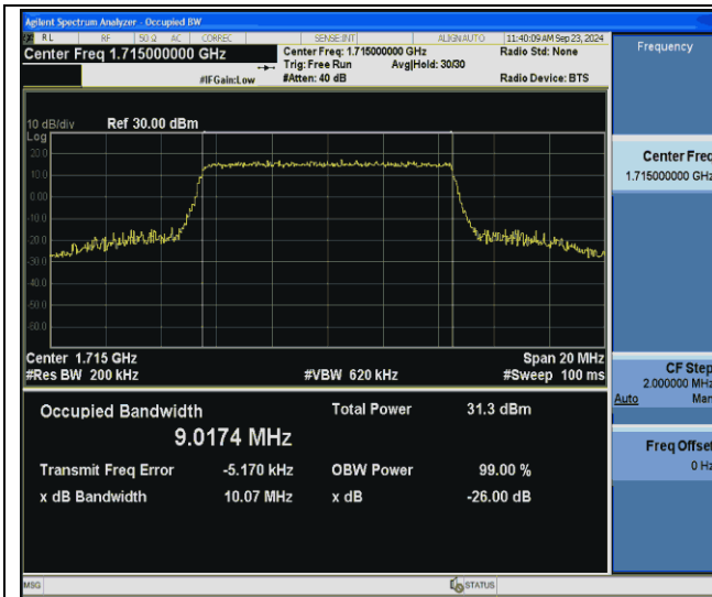
Band66-10MHz-64QAM-132022-50RB#0-PASS
