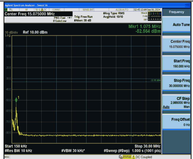
Band66-20MHz-QPSK-132572-1RB#0-0.15~30-PASS
