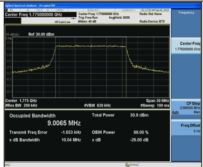
Band66-10MHz-16QAM-132622-50RB#0-PASS
