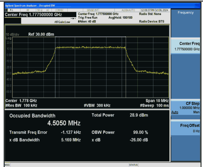
Band66-5MHz-256QAM-132647-25RB#0-PASS
