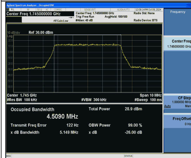
Band66-5MHz-256QAM-132322-25RB#0-PASS
