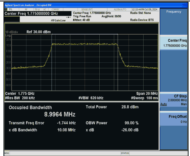
Band66-10MHz-256QAM-132622-50RB#0-PASS
