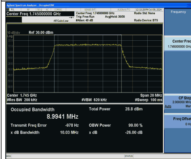
Band66-10MHz-256QAM-132322-50RB#0-PASS
