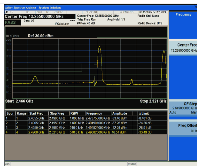
41-41-15MHz-10MHz-QPSK@QPSK-QPSK@QPSK-39725- 39845-1RB#0@75RB#0-1RB#49@50RB#0-PASS
