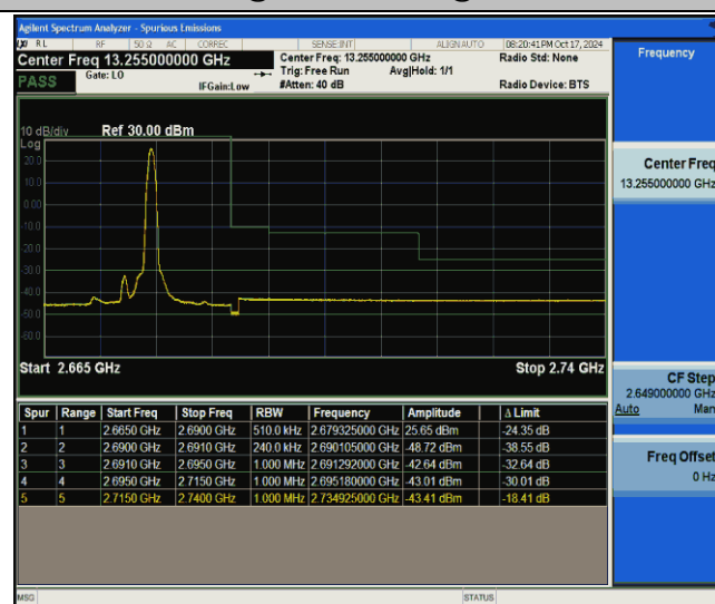
41-41-15MHz-10MHz-QPSK@QPSK-QPSK@QPSK-41417-41537-1RB#74@75RB#0-0RB#0@50RB#0-PASS
