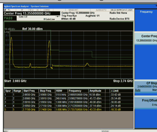
41-41-15MHz-10MHz-QPSK@QPSK-QPSK@QPSK-41417-41537-1RB#0@75RB#0-1RB#49@50RB#0-PASS
