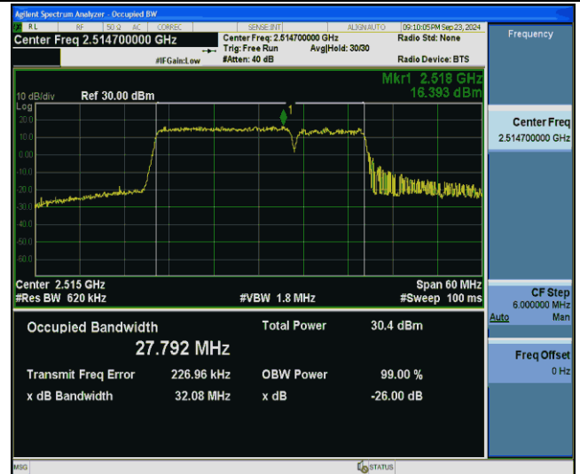
7-7-20MHz-10MHz-16QAM-16QAM-20850-20994-100RB#0- 50RB#0-PASS
