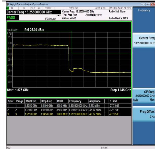
NTNV-n2-PC3-15-35-H-DFT-PI2BPSK-Outer_Full-PASS
