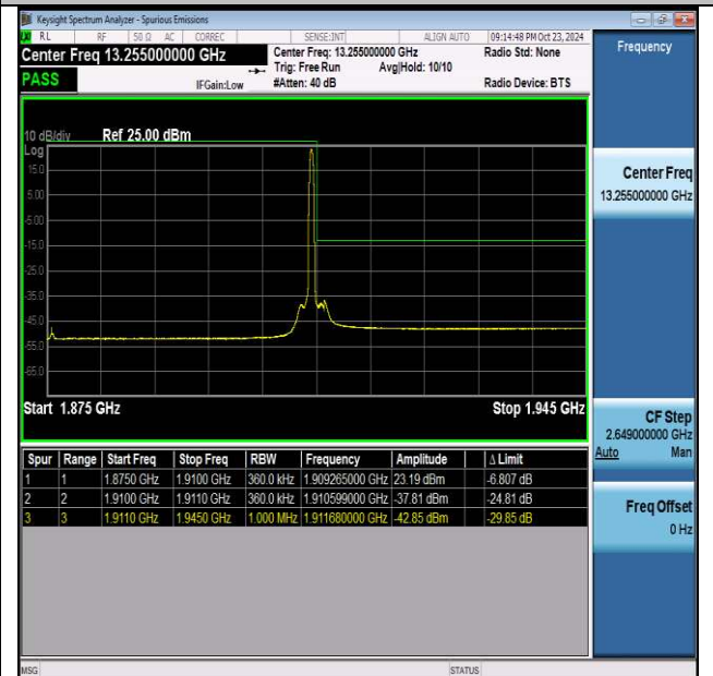
NTNV-n2-PC3-15-35-H-DFT-PI2BPSK-Edge_1RB_Right-PASS
