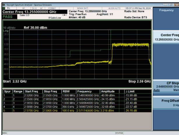
NTNV-n38-PC3-30-20-L-DFT-BPSK-Outter_Full-PASS
