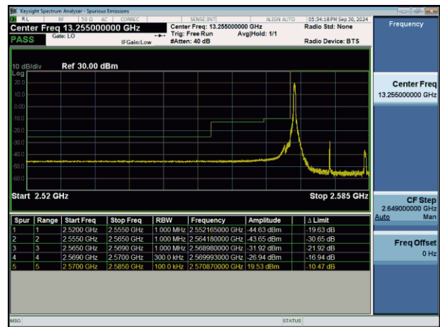
NTNV-n38-PC3-30-15-L-DFT-BPSK-Edge_1RB_Left-PASS
