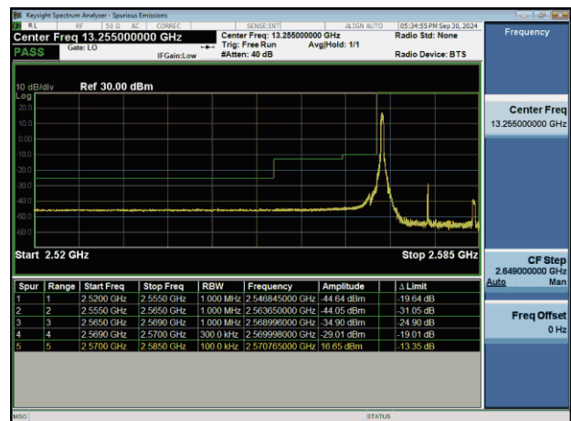
NTNV-n38-PC3-30-15-L-CP-QPSK-Edge_1RB_Left-PASS
