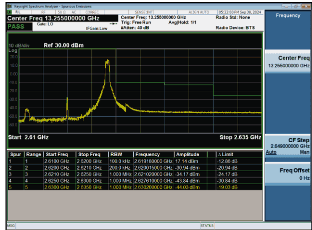
NTNV-n38-PC3-30-10-H-CP-QPSK-Edge_1RB_Right-PASS
