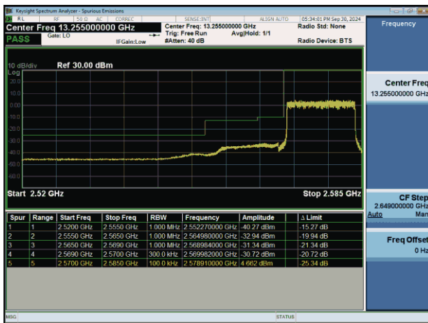
NTNV-n38-PC3-30-15-L-DFT-BPSK-Outet_Full-PASS
