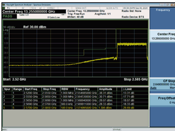
NTNV-n38-PC3-30-15-L-CP-QPSK-Outet_Full-PASS
