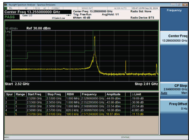
NTNV-n38-PC3-30-40-L-DFT-BPSK-Edge_1RB_Left-PASS
