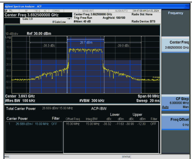
Band48-15MHz-QPSK-56665-75RB#0-PASS
