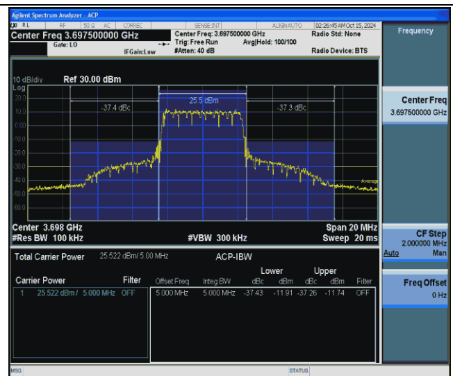
Band48-5MHz-QPSK-56715-25RB#0-PASS
