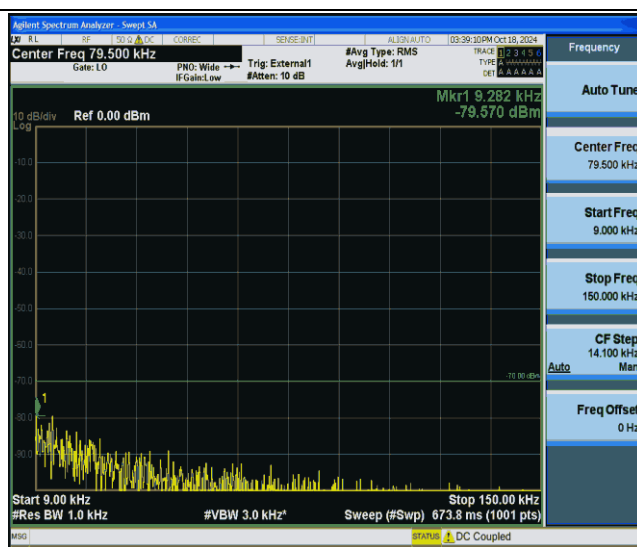
Band48-20MHz-QPSK-55990-1RB#0-0.009~0.15-PASS
