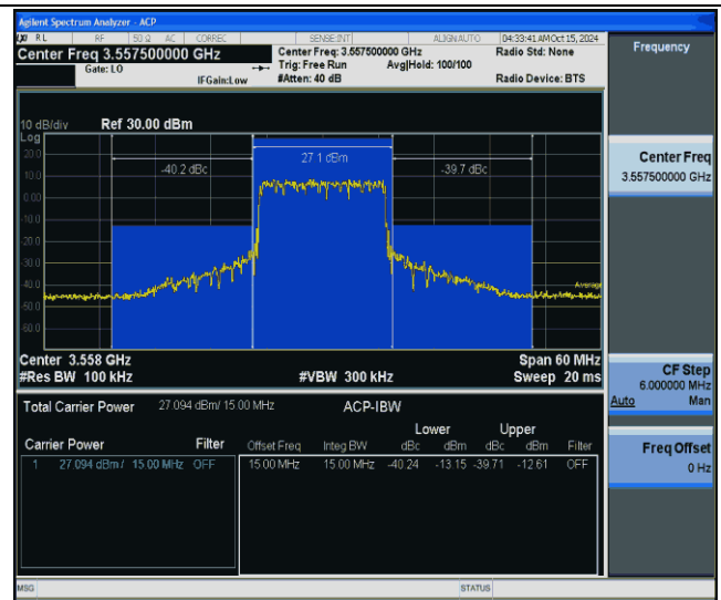
Band48-15MHz-QPSK-55315-75RB#0-PASS
