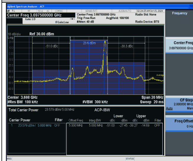
Band48-5MHz-QPSK-56715-1RB#24-PASS
