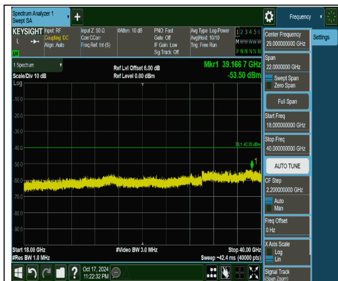
Band48-20MHz-QPSK-55340-1RB#0-18000~40000-PASS
