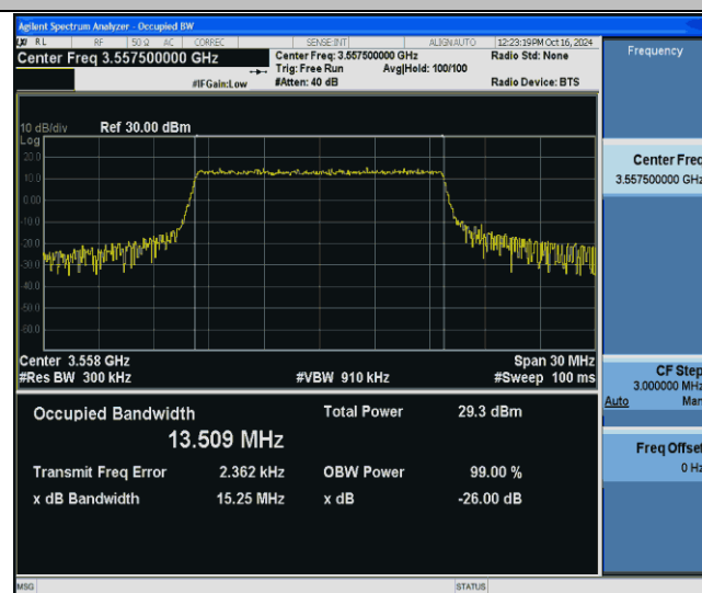
Band48-15MHz-256QAM-55315-75RB#0-PASS
