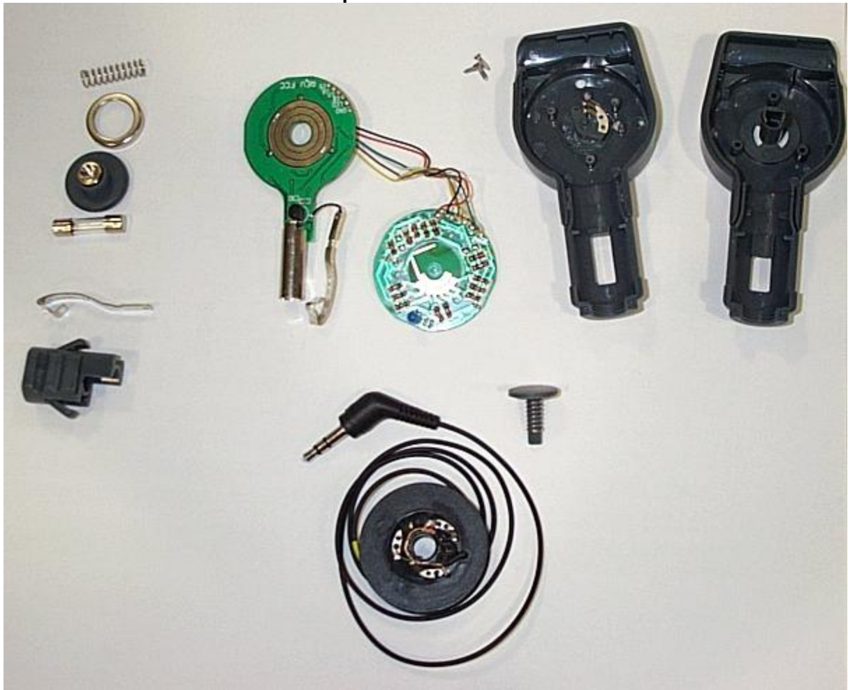
Exploded View of EUT
