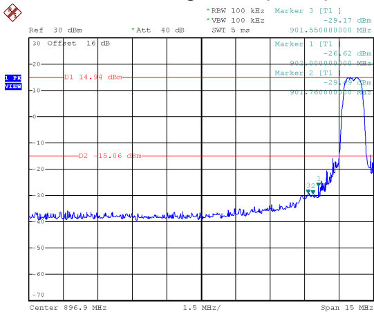
Bandedge CH03 (Lower)
