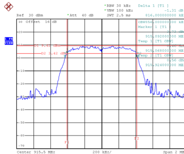
CH27 6 dB Bandwidth
