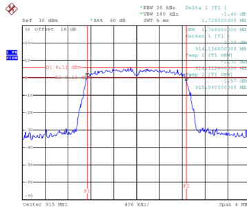
CH26 6 dB Bandwidth
