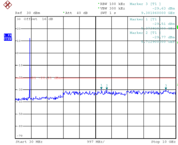
CH49 – 10th Harmonic of the fundamental frequency
