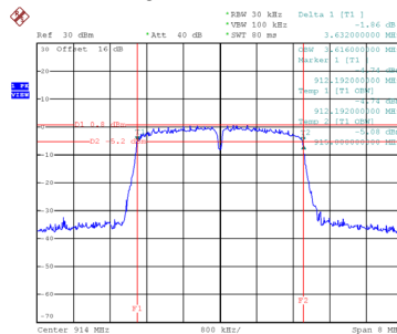
CH24 6 dB Bandwidth
