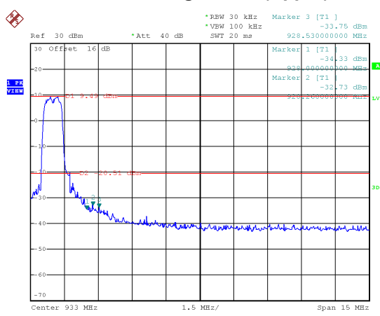
Bandedge CH49 (Upper)
