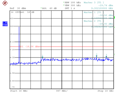
CH27 – 10th Harmonic of the fundamental frequency
