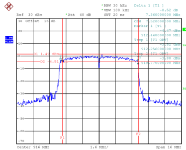
CH28 6 dB Bandwidth
