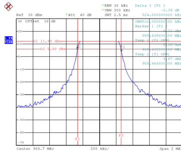
908.7MHz 6 dB Bandwidth
