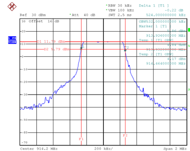
914.2MHz
