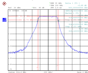
914.9MHz 6 dB Bandwidth
