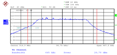
914.9MHz
