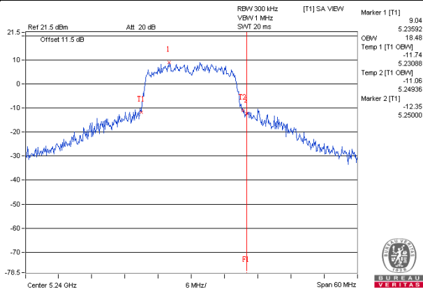
802.11n (20MHz) / Chain 0 – CH48
