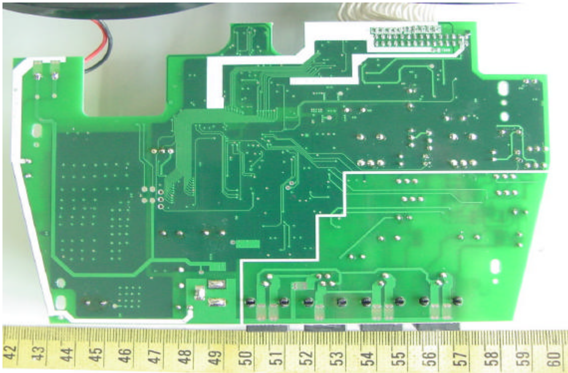
Solder View of Base Unit 's PCB
