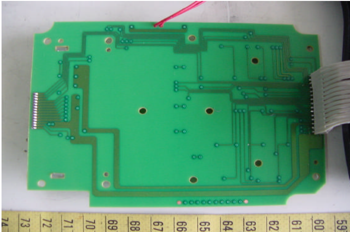
Solder View of Base Unit 's Main PCB
