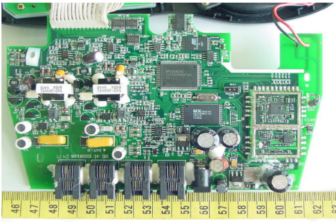
Component View of Base Unit 's PCB
