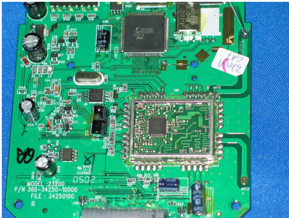
Docking Station Oscillator PCB comp side
