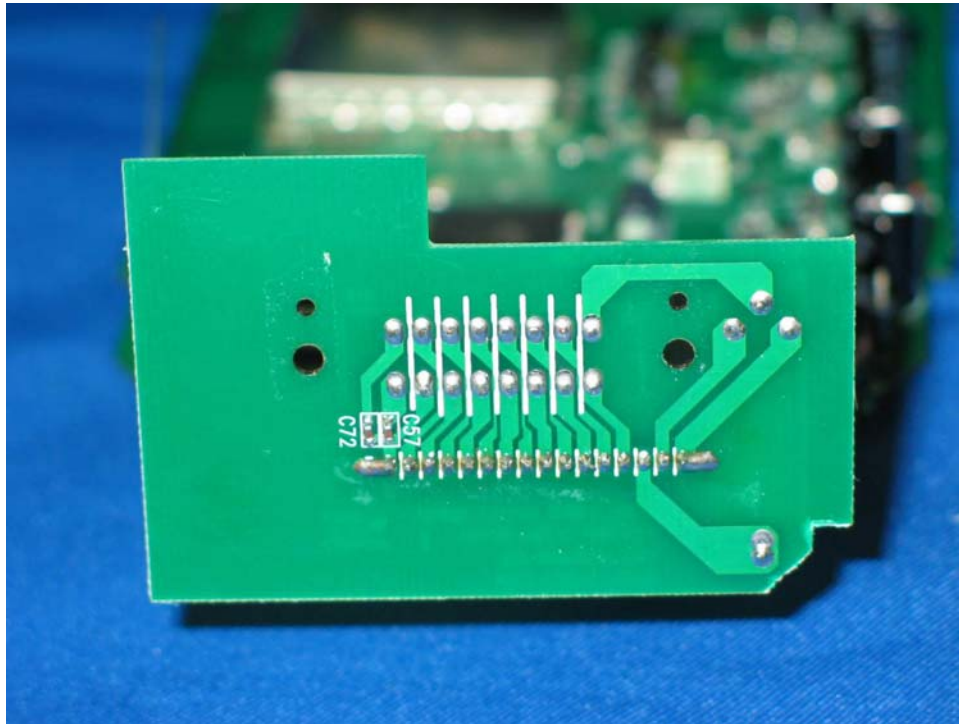
Docking Station connector PCB rear side
