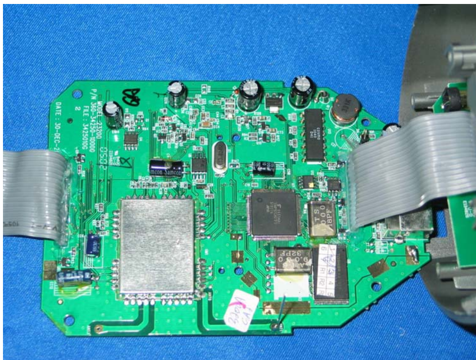
Docking Station Main PCB comp side (View 1)
