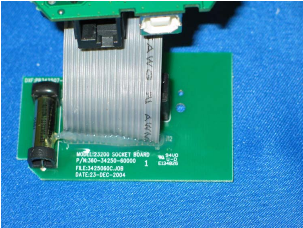
Docking Station connector PCB front side (View 2)
