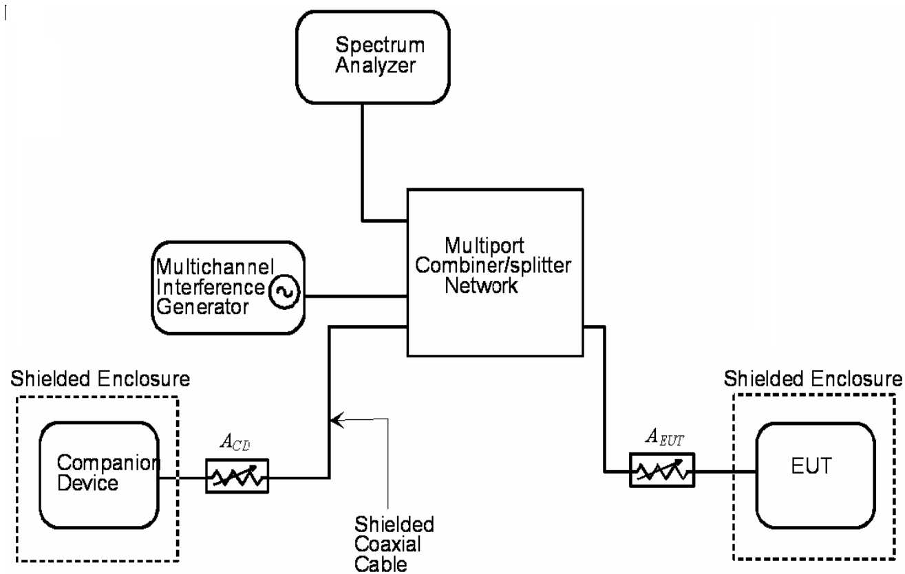
Test Set-Up 5 This test setup is used for all Monitoring and Time and Spectrum Access Procedure tests.
