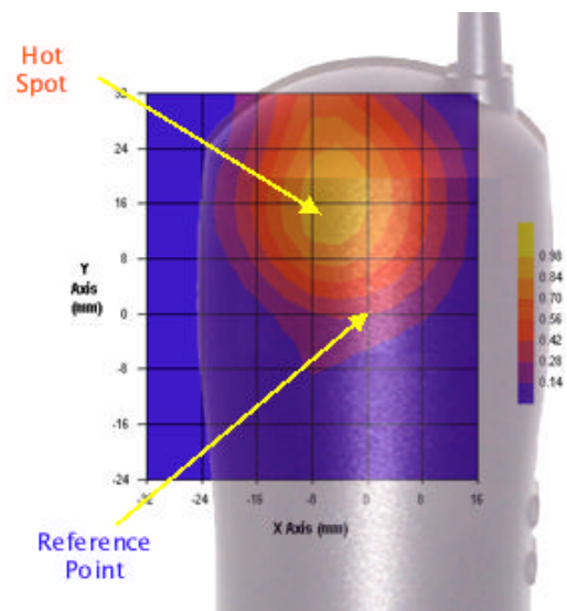
(Rear View)
